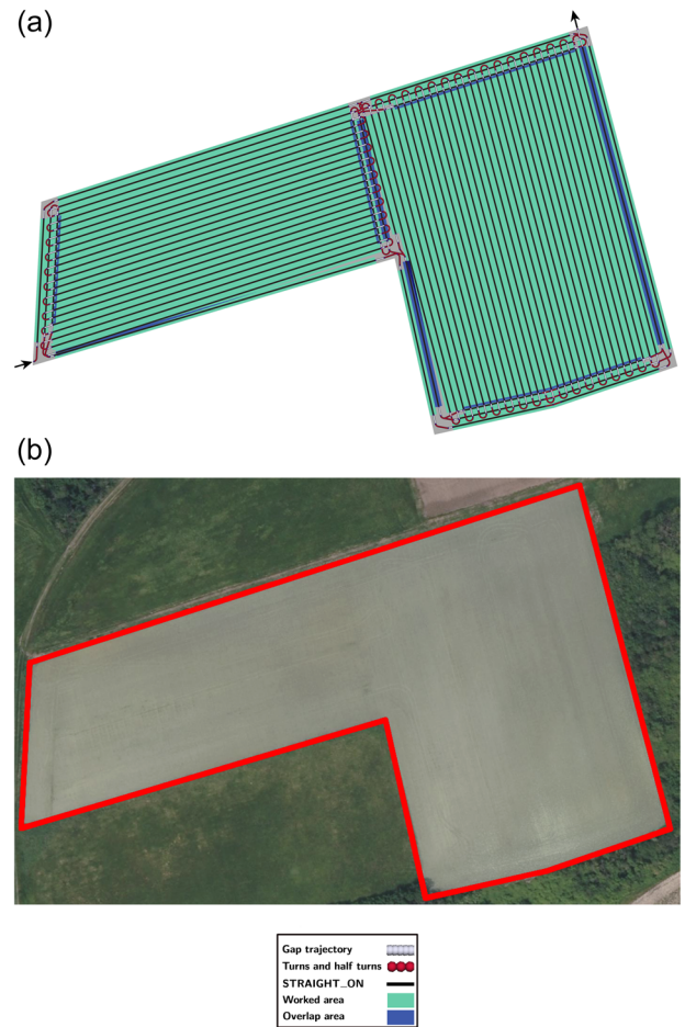
FIGURE A31 Black arrows indicate where the robot enters and exits. (a) Most optimal and similar result and (b) satellite image. [Color figure can be viewed at wileyonlinelibrary.com ]
