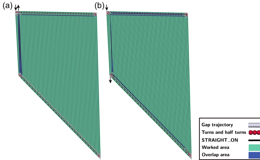
FIGURE 8 Most optimal solutions for Field S7 while considering it is only accessible from its upper edge (a) or from all its edges (b). Black arrows indicate where the robot enters and exits. (a) S7—one accessible edge and (b) S7—all edges are accessible. [Color figure can be viewed at wileyonlinelibrary.com ]
