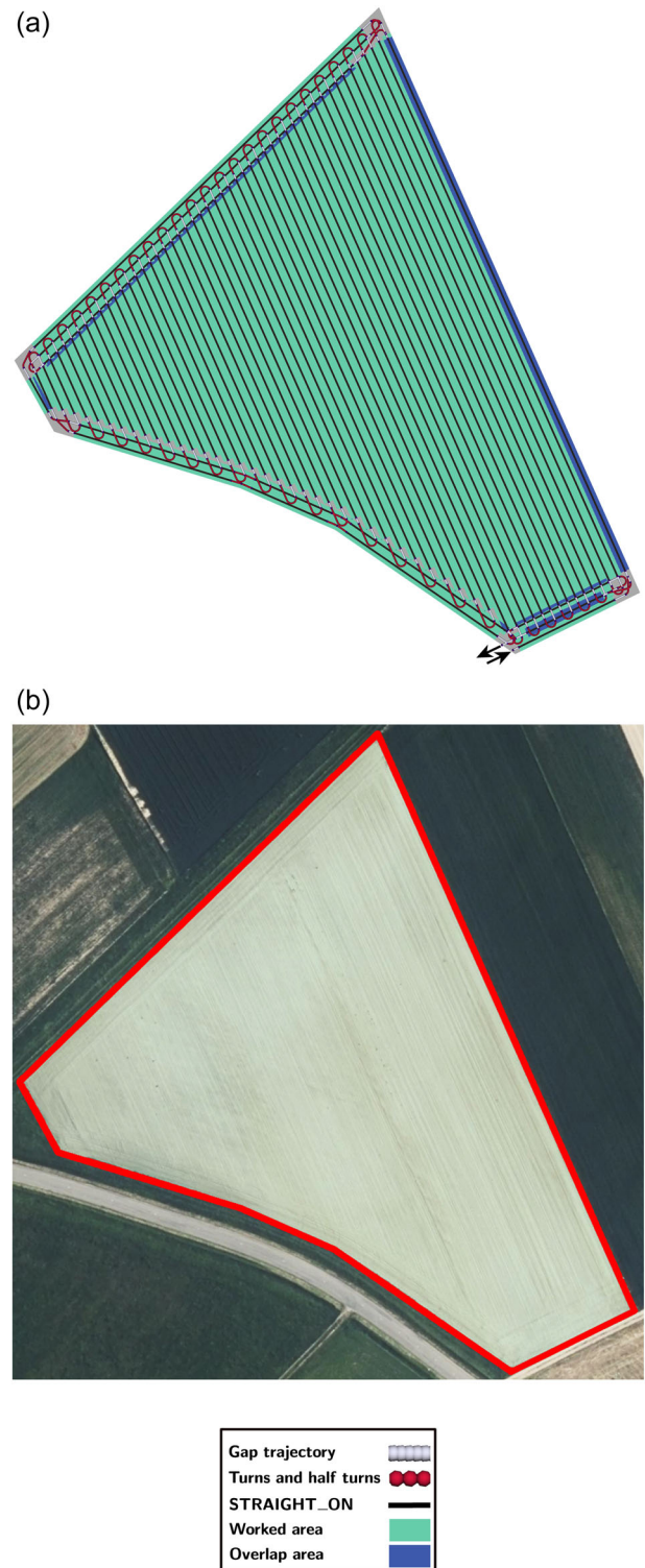
FIGURE A16 Black arrows indicate where the robot enters and exits. (a) Most optimal and similar result and (b) satellite image. [Color figure can be viewed at wileyonlinelibrary.com ]
