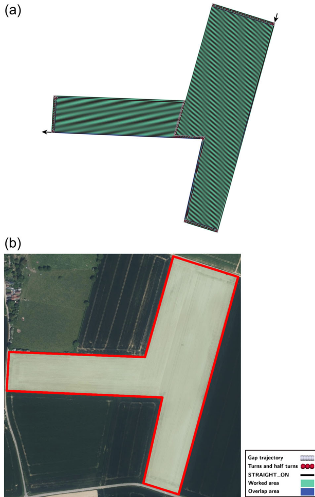
FIGURE A28 Black arrows indicate where the robot enters and exits. (a) Most optimal and similar result and (b) satellite image. [Color figure can be viewed at wileyonlinelibrary.com ]
