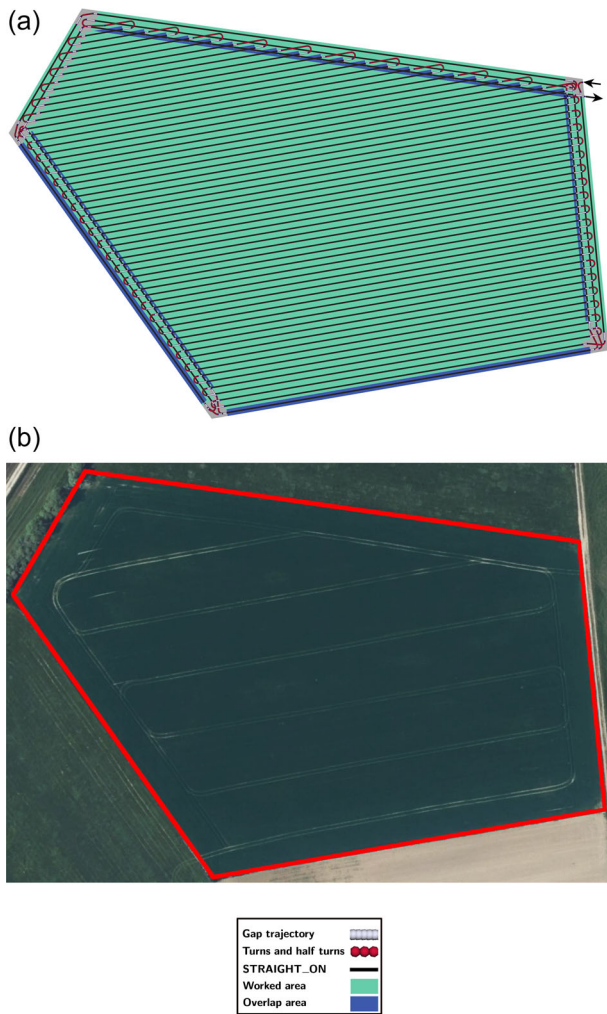
FIGURE A3 Black arrows indicate where the robot enters and exits. (a) Most optimal and similar result and (b) satellite image. [Color figure can be viewed at wileyonlinelibrary.com ]
