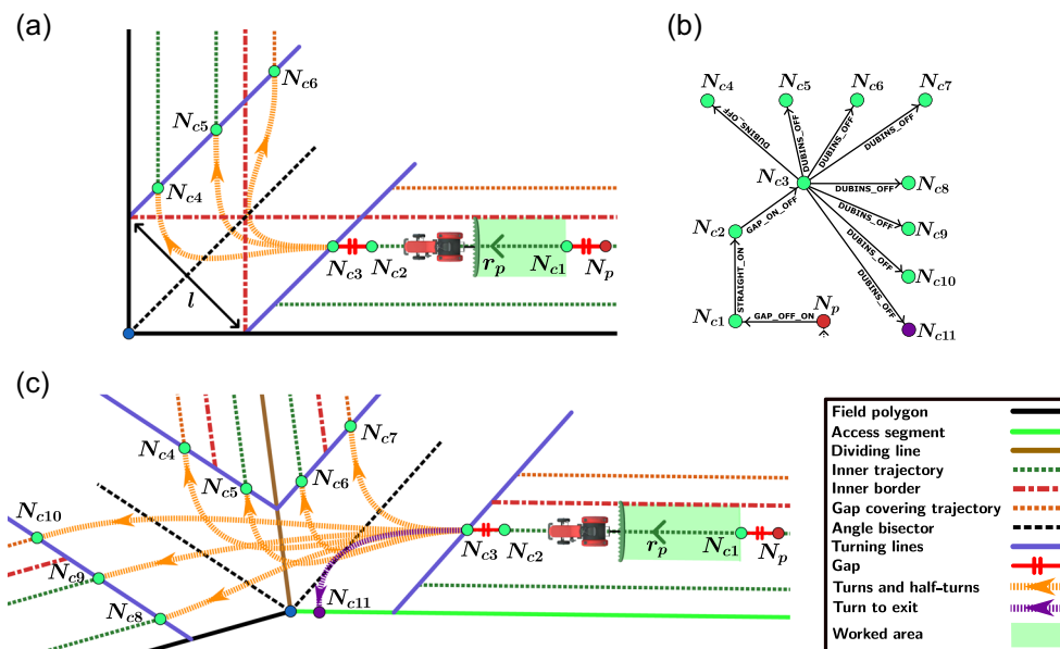
FIGURE 2 Trajectory (a, c) and tree (b) representations of turns inside the turning spaces. (b) The tree representation of trajectories of (c). [Color figure can be viewed at wileyonlinelibrary.com ]
