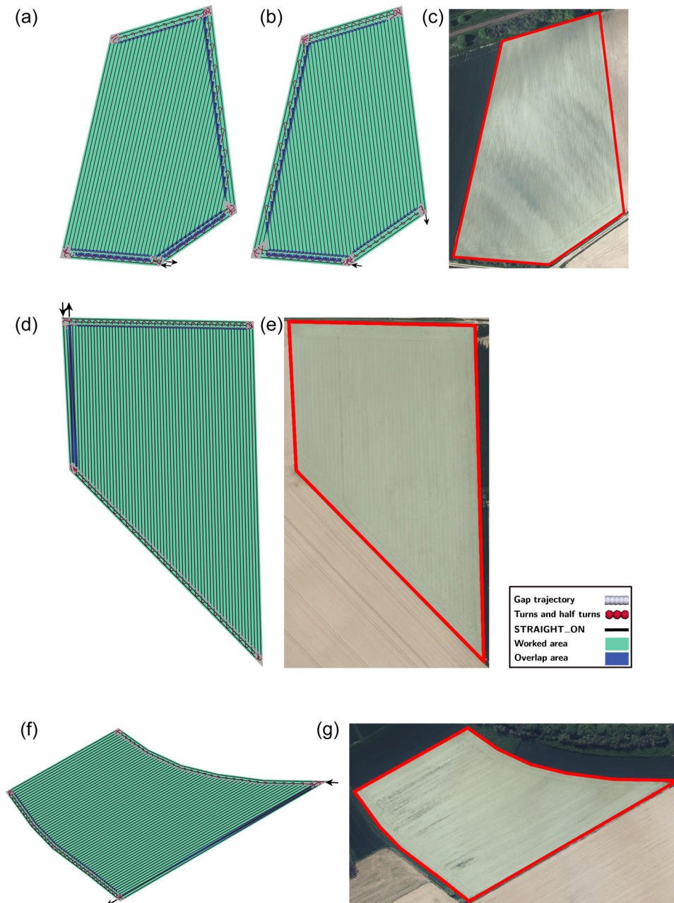
FIGURE 6 Obtained results on six fields from the data set and their reference satellite image. Black arrows indicate where the robot enters and exits. (a) S6—most optimal solution, (b) S6—most similar solution, (c) S6—satellite image, (d) S7—most optimal and similar solution, (e) S7—satellite image, (f) S8—most optimal and similar solution, (g) S8—satellite image, (h) S9—most optimal and similar solution, (i) S9—satellite image, (j) C4—most optimal solution, (k) C4—satellite image, (l) C2—most optimal solution, (m) C2—most similar solution, and (n) C2—satellite image. [Color figure can be viewed at wileyonlinelibrary.com ]
