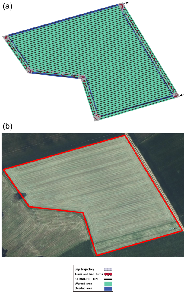
FIGURE A11 Black arrows indicate where the robot enters and exits. (a) Most optimal and similar result and (b) Satellite image. [Color figure can be viewed at wileyonlinelibrary.com ]
