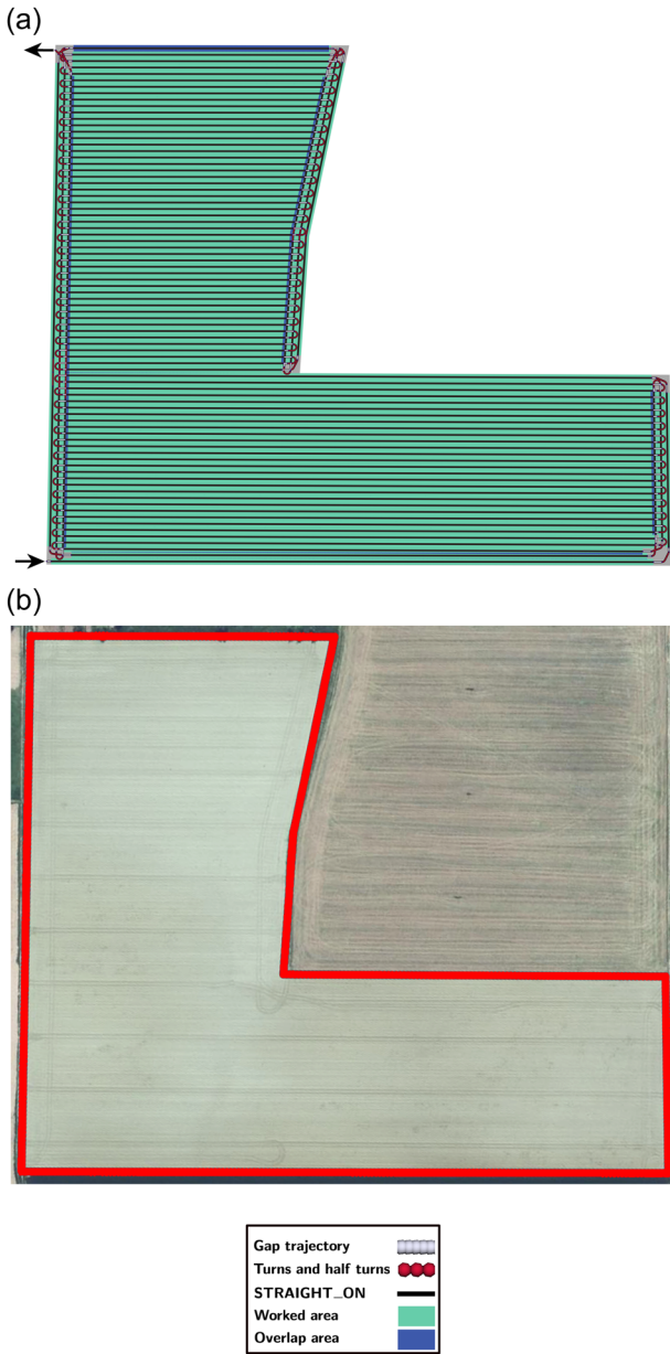
FIGURE A25 Black arrows indicate where the robot enters and exits. (a) Most optimal and similar result and (b) satellite image. [Color figure can be viewed at wileyonlinelibrary.com ]
