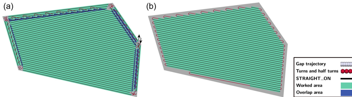
FIGURE 10 Result obtained on Field S6 from the data set using our approach and F2C. (a) S6—our approach and (b) S6—F2C. [Color figure can be viewed at wileyonlinelibrary.com ]
