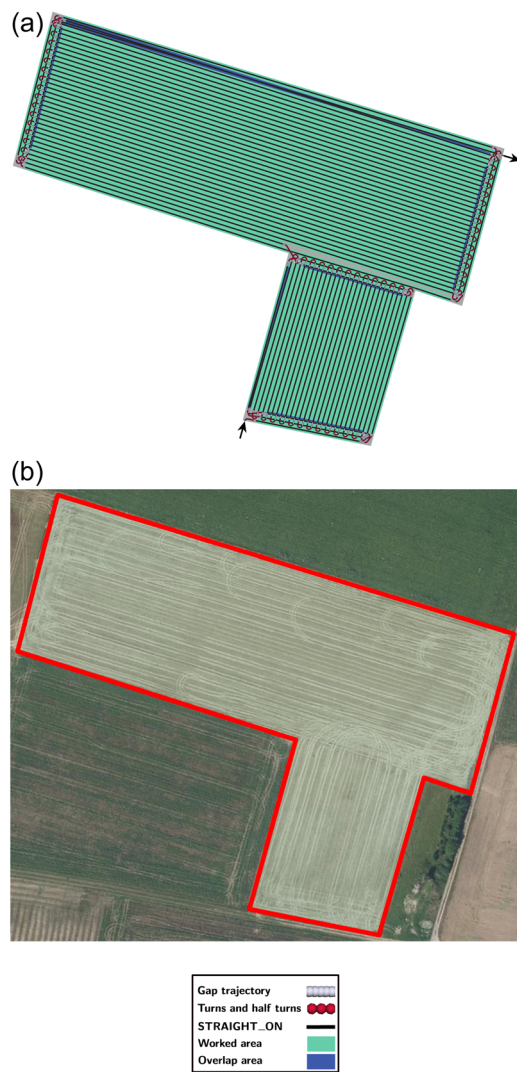
FIGURE A32 Black arrows indicate where the robot enters and exits. (a) Most optimal and similar result and (b) satellite image. [Color figure can be viewed at wileyonlinelibrary.com ]
