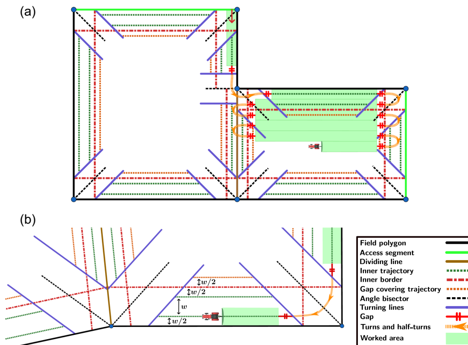
FIGURE 1 Preprocessing result for p = 2 . The field polygon is represented by blue points and black and green solid segments. (a) Preprocessing result for a field and (b) a close-up on a preprocessing result. [Color figure can be viewed at wileyonlinelibrary.com ]
