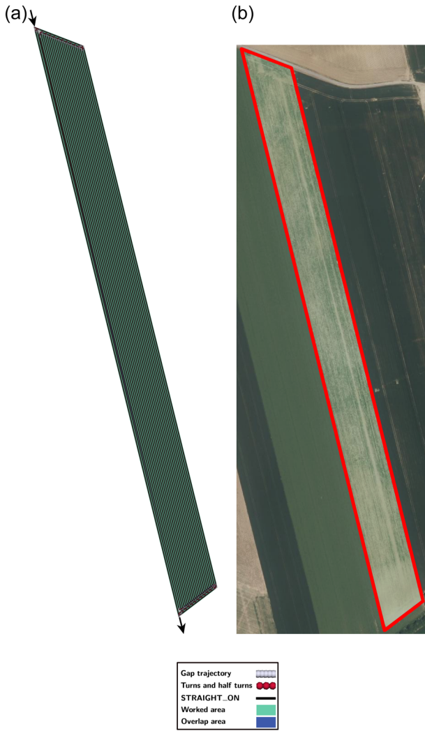
FIGURE A5 Black arrows indicate where the robot enters and exits. (a) Most optimal and similar result and (b) satellite image. [Color figure can be viewed at wileyonlinelibrary.com ]
