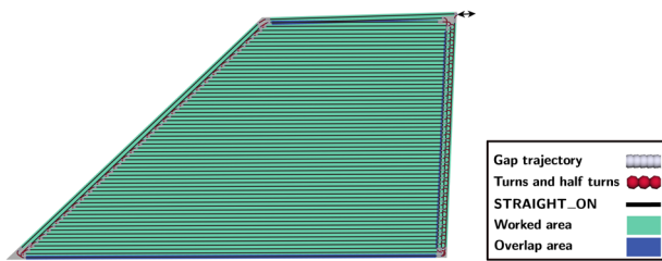
FIGURE 9 Most optimal solutions for Field S7 when \gamma_{off} was set to 2m. Black arrows indicate where the robot enters and exits. [Color figure can be viewed at wileyonlinelibrary.com ]
