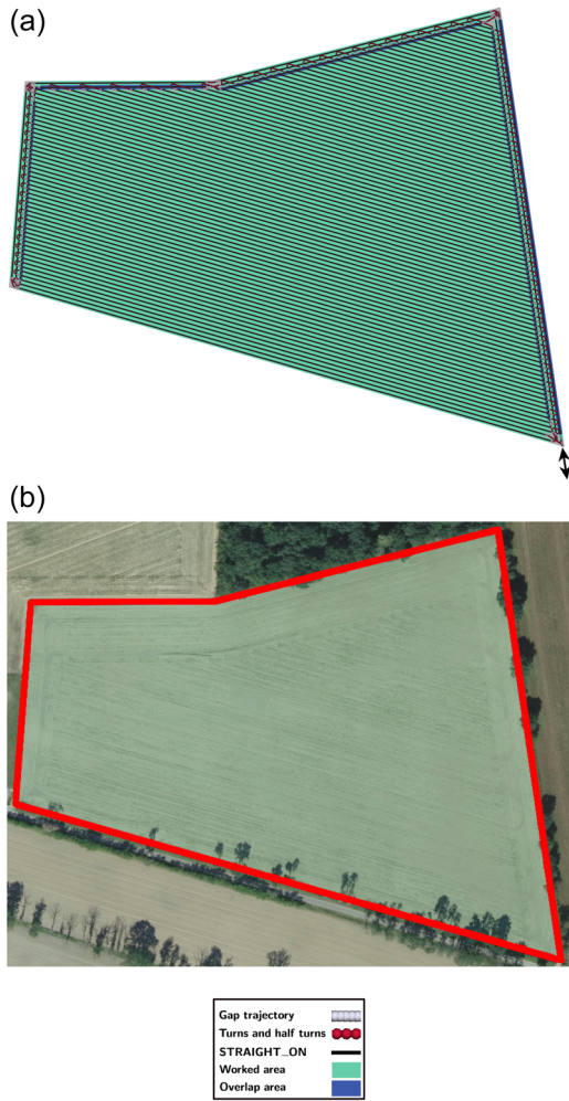
FIGURE A13 Black arrows indicate where the robot enters and exits. (a) Most optimal and similar result and (b) satellite image. [Color figure can be viewed at wileyonlinelibrary.com ]
