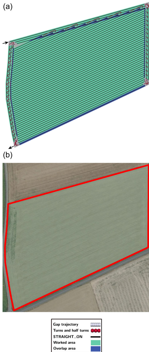
FIGURE A19 Black arrows indicate where the robot enters and exits. (a) Most optimal and similar result and (b) satellite image. [Color figure can be viewed at wileyonlinelibrary.com ]
