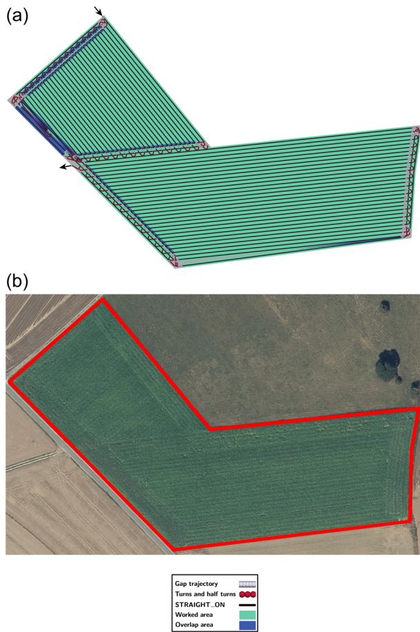
FIGURE A23 Black arrows indicate where the robot enters and exits. (a) Most optimal result and (b) satellite image. [Color figure can be viewed at wileyonlinelibrary.com ]
