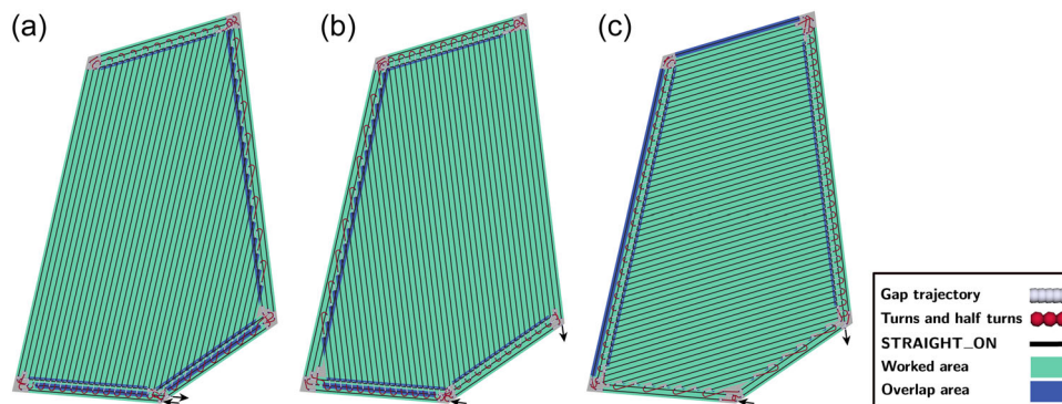
FIGURE 7 Most optimal solution for different families for Field S6. Black arrows indicate where the robot enters and exits. (a) S6—first family, (b) S6—second family, and (c) S6—third family. [Color figure can be viewed at wileyonlinelibrary.com ]
