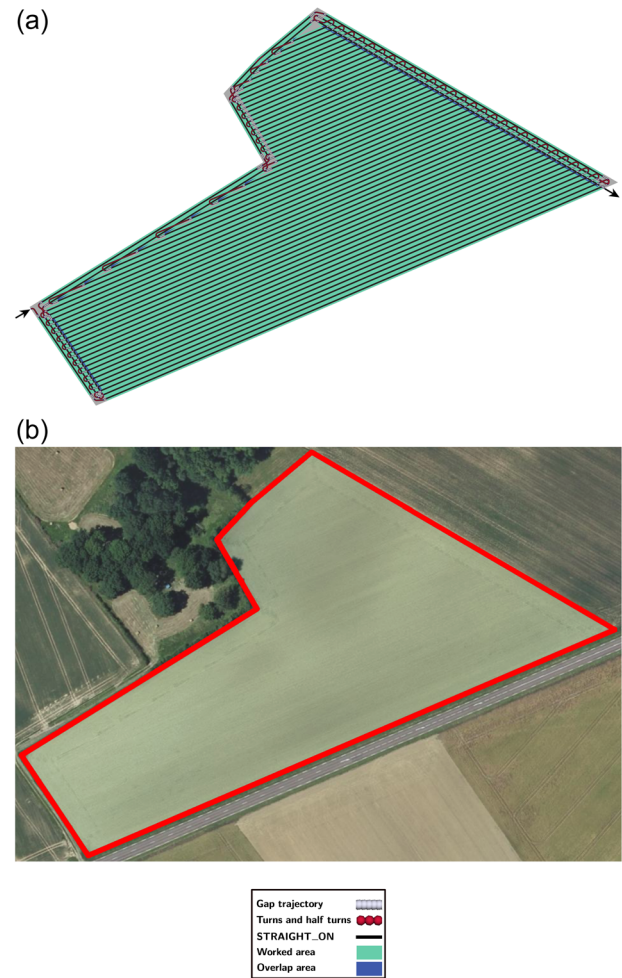
FIGURE A29 Black arrows indicate where the robot enters and exits. (a) Most optimal and similar result and (b) satellite image. [Color figure can be viewed at wileyonlinelibrary.com ]
