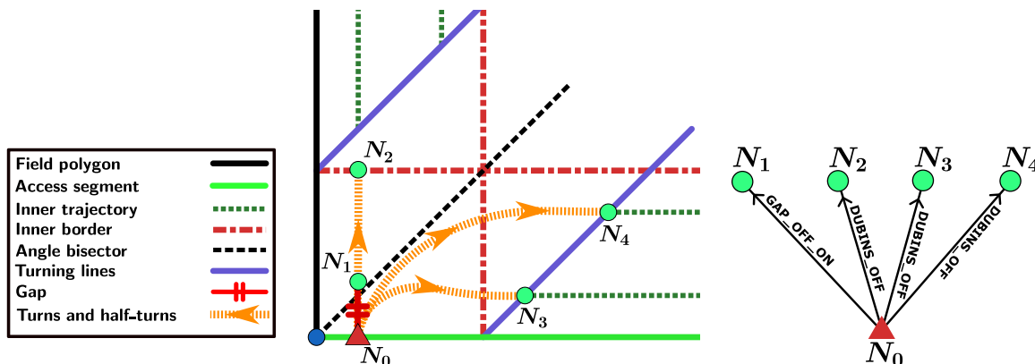
FIGURE 3 Trajectory and tree representation of the initialization. The entrance and root of the tree N_0 are represented by a red triangle. N_1, N_2, N_3, and N_4 are the first nodes that might be added to the tree as children of N_0 . Orange dashed lines represent trajectories from N_0 toward its children. [Color figure can be viewed at wileyonlinelibrary.com ]
