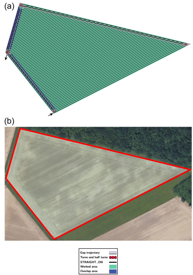
FIGURE A22 Black arrows indicate where the robot enters and exits. (a) Most optimal and similar result and (b) satellite image. [Color figure can be viewed at wileyonlinelibrary.com ]
