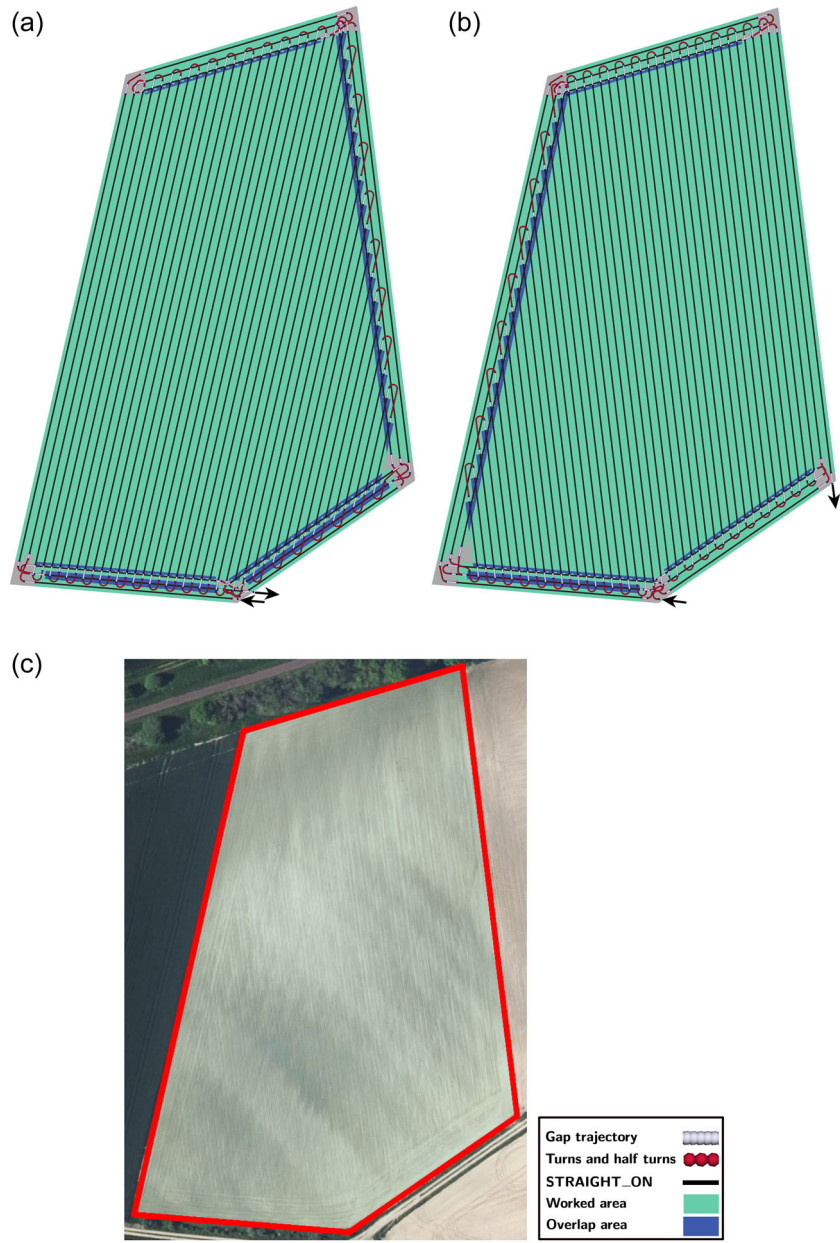
FIGURE A8 Black arrows indicate where the robot enters and exits. (a) Most optimal result, (b) most similar result, and (c) satellite image. [Color figure can be viewed at wileyonlinelibrary.com ]
