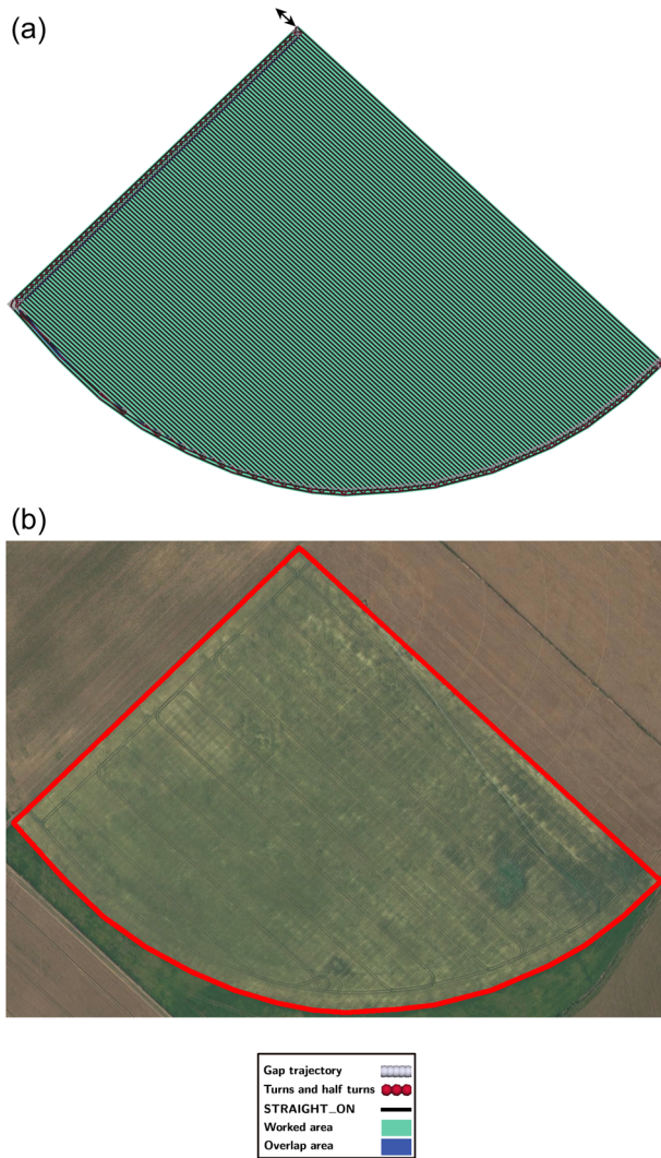
FIGURE A17 Black arrows indicate where the robot enters and exits. (a) Most optimal and similar result and (b) satellite image. [Color figure can be viewed at wileyonlinelibrary.com ]
