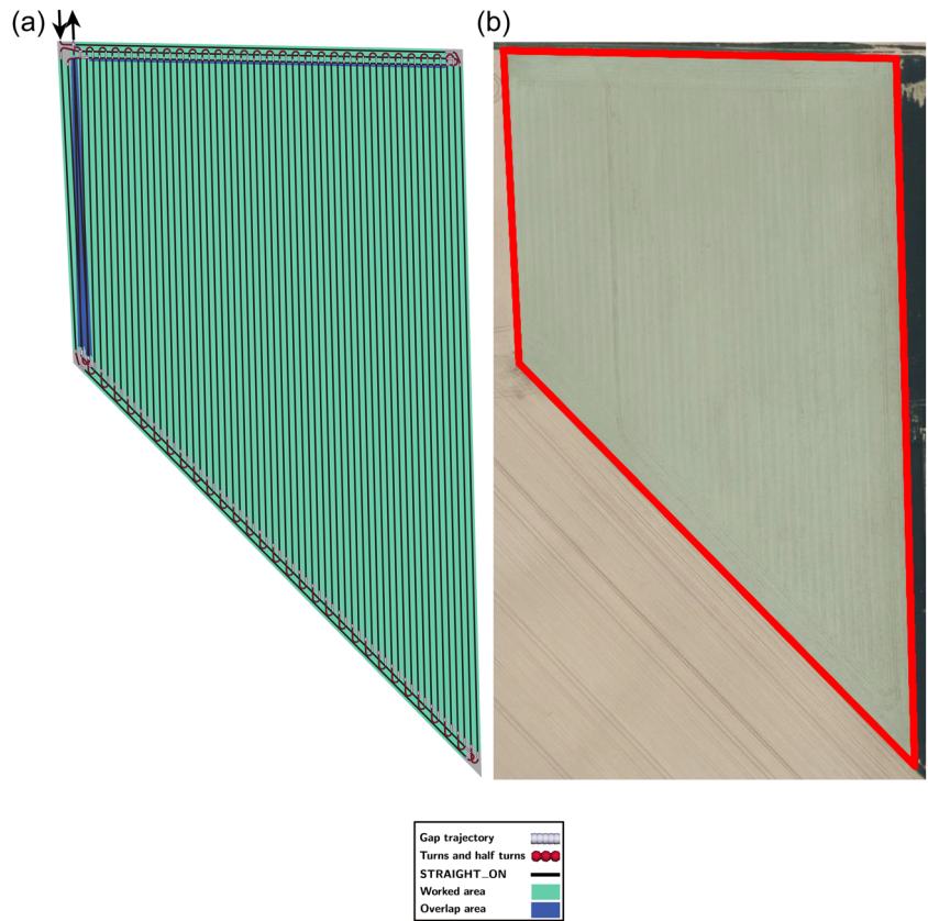
FIGURE A9 Black arrows indicate where the robot enters and exits. (a) Most optimal and similar result and (b) satellite image. [Color figure can be viewed at wileyonlinelibrary.com ]
