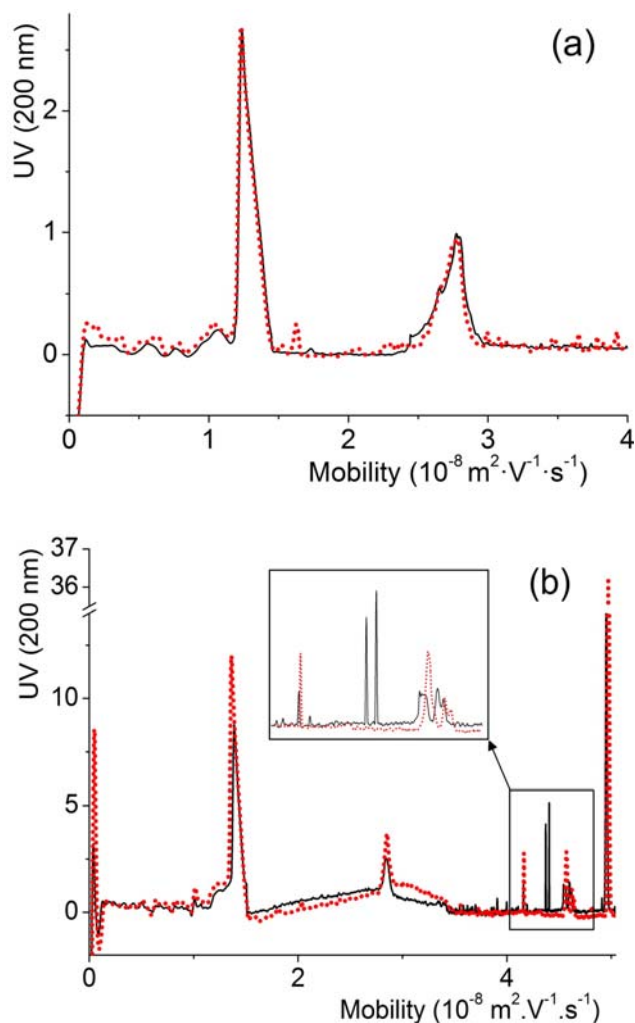
Fig. 10. Comparison of gellan gum before and after sonication (solid black line and dotted red line, respectively): (a) LAEFGG (samples LAEFGG and LAEFGG-Son, first injections series), (b) HAGG (samples HAGG and HAGG-Son, third injections series).
