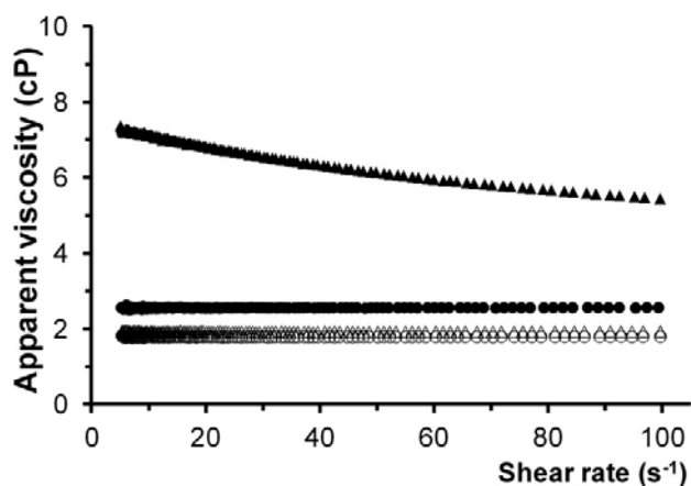
Fig. 9. The apparent viscosity of as-prepared (full symbols) and sonicated (empty symbols) solutions of 0.5 g·L -1 of LAGG (circles) and HAGG (triangles) in water.
