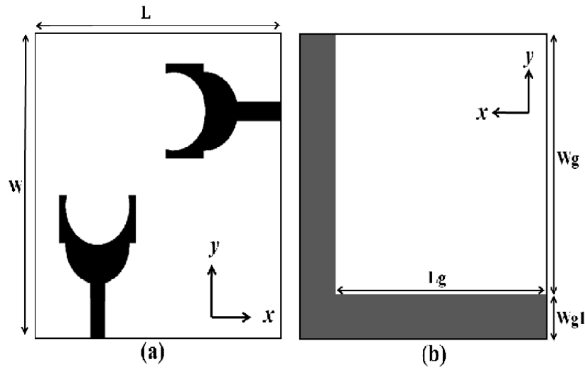
Figure 4. Proposed UWB MIMO antenna: (a) front view, (b) rear view Optimized dimensions: L=45 \text{ mm} , W=45 \text{ mm} , L_g=38.5 \text{ mm} , W_g=38.5 \text{ mm} , W_{g1}=6.5 \text{ mm}
