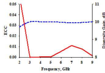
Figure 11. Simulated ECC and diversity gain of the proposed antenna
