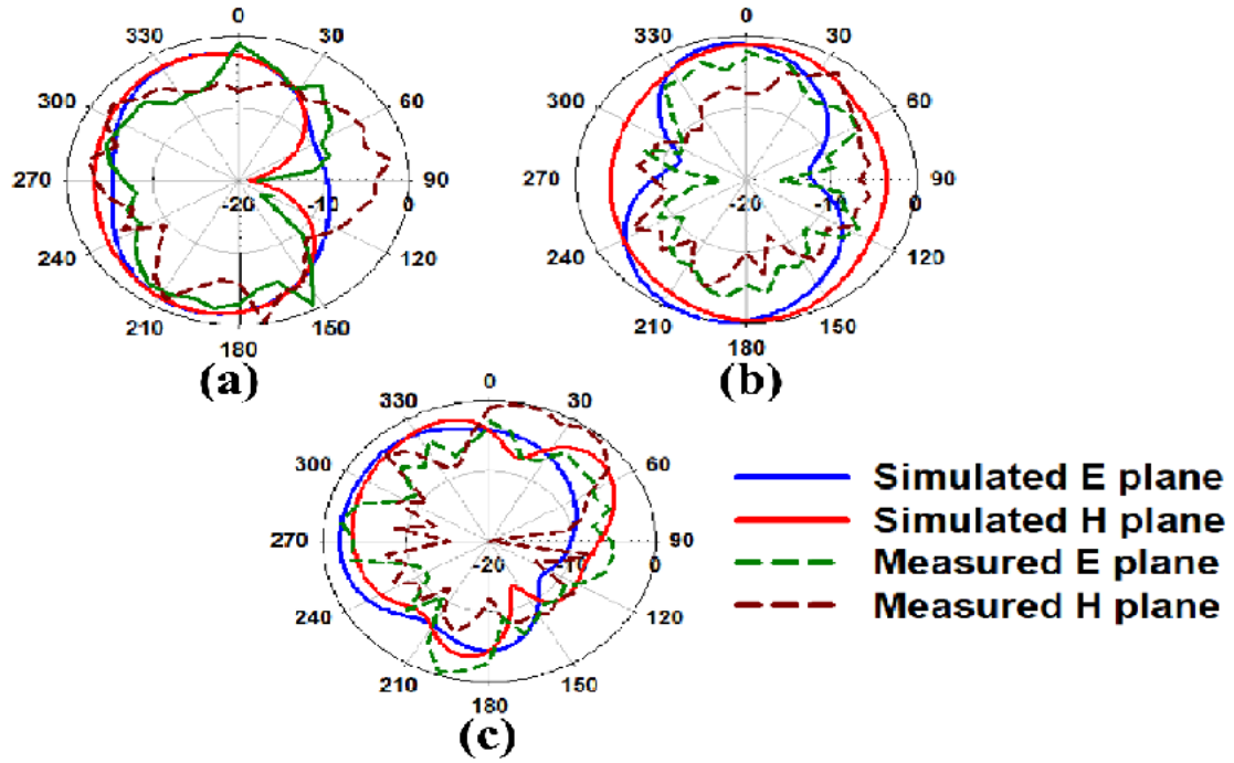
Figure 9. Simulated and measured normalized radiation pattern at port 1 (a) 3 GHz, (b) 5 GHz, and (c) 7 GHz
