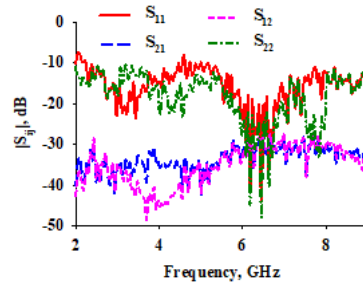
Figure 8. Measured reflection and isolation coefficients characteristics of UWB MIMO antenna
