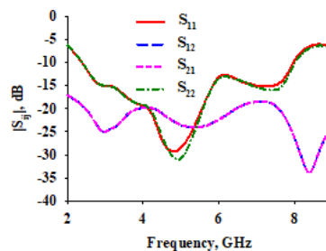
Figure 5. Simulated reflection and isolation coefficients characteristics of UWB MIMO antenna
