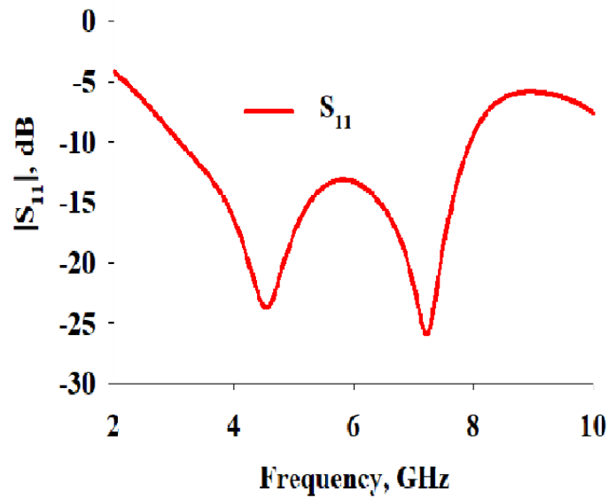
Figure 3. Reflection coefficients characteristics of a single element UWB antenna
