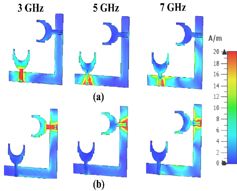
Figure 6. Surface current distribution of the UWB MIMO antenna at 3, 5, and 7 GHz with (a) port 1 excited and (b) port 2 excited
