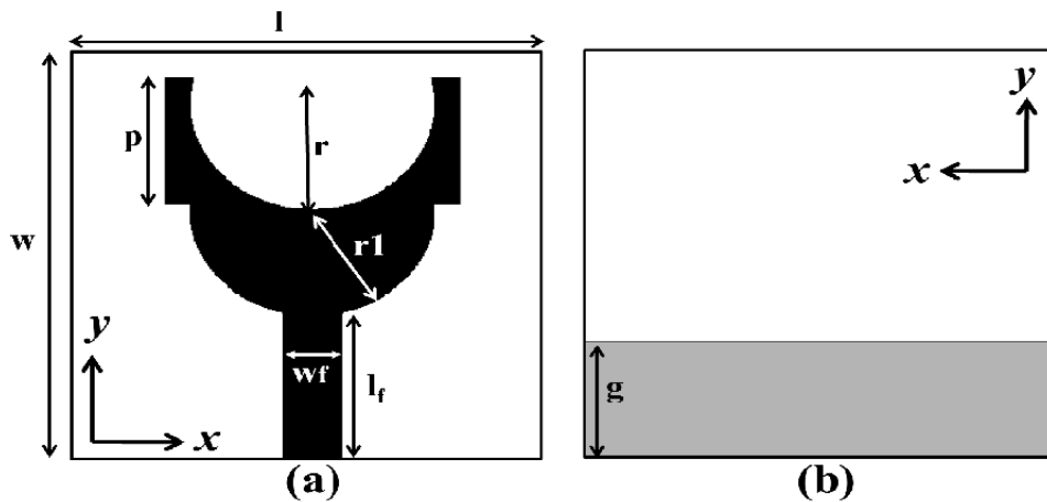
Figure 1. Proposed single element UWB antenna: (a) front view (b) rear view Optimized dimensions: l=22.5 mm w=22.5 mm, p=7 mm, r=5.8 mm, r1=5.8 mm l_f =8 mm, wf=2.8 mm, g=6.5 mm
