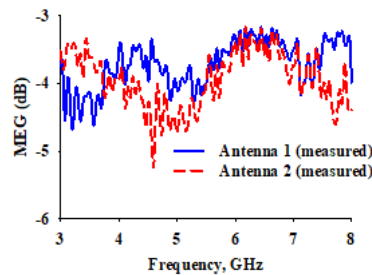
Figure 12. Measured MEG (dB) of the proposed antenna
