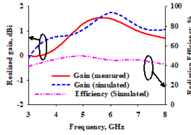
Figure 10. Simulated and measured realized gain and simulated efficiency of the proposed MIMO antenna
