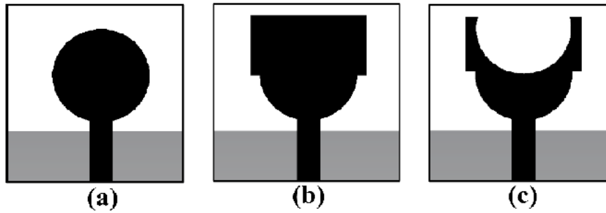
Figure 2. Evolution of a single element UWB antenna: (a) evolution 1, (b) evolution 2, and (c) proposed antenna
