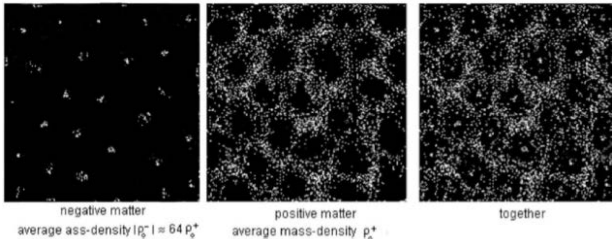
Fig.4 : Evolution when |\rho^{(-)}| \gg \rho^{(+)}
