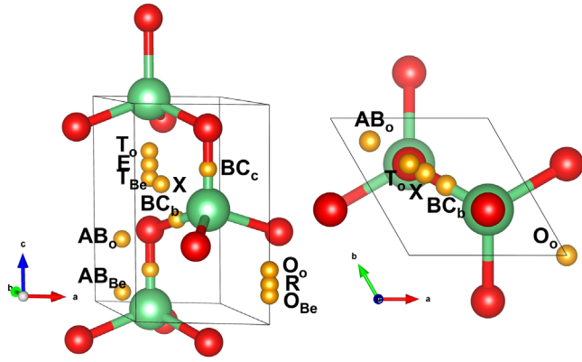
FIGURE 1 (Color online) Schematic representation of the BeO structure: Be and O atoms are in green and red, respectively. Gold balls represent the interstitial hydrogen sites considered here. The figure on the left (right) is a lateral (top sliced) view of the primitive cell. Figures were built with VESTA. 30
