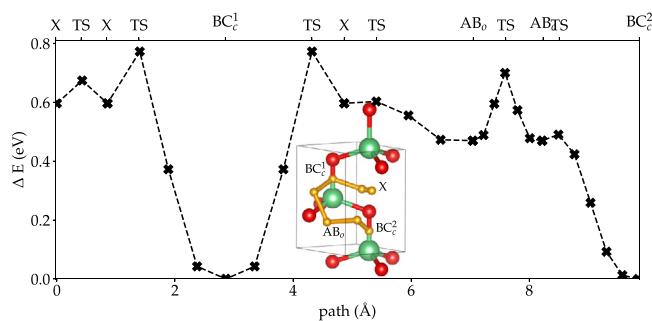
FIGURE 9 (Color online) Energy profile computed with the PBE functional and diagram of the migration path of H^+ between stable sites. The identified hydrogen paths are drawn in gold and red (green) balls correspond to oxygen (beryllium) atoms. PBE, Perdew–Burke–Ernzerhof.
