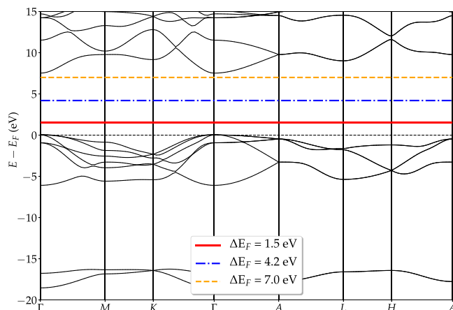
FIGURE 2 Electronic band structure of the BeO wurtzite (PBE functional) along high symmetry points of the first Brillouin zone. The Fermi level was set at the top of the valence band, and \Delta E_F = E_F - E_{\text{vbm}} . The 4.2 eV value (blue line) corresponds to a shift of the Fermi level position induced by the assumption of the electrically neutral system for charged hydrogen solubility, whereas the other values (red and orange lines) are selected for the illustrative solubility calculations. PBE, Perdew–Burke–Ernzerhof.
