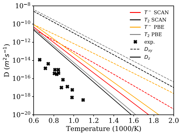
FIGURE A.2 (Color online) Diffusion coefficients of T^- and T_2 computed with PBE and SCAN functionals. Experimental data were extracted from Ref. [12]. PBE, Perdew–Burke–Ernzerhof; SCAN, strongly constrained and appropriately normed.
