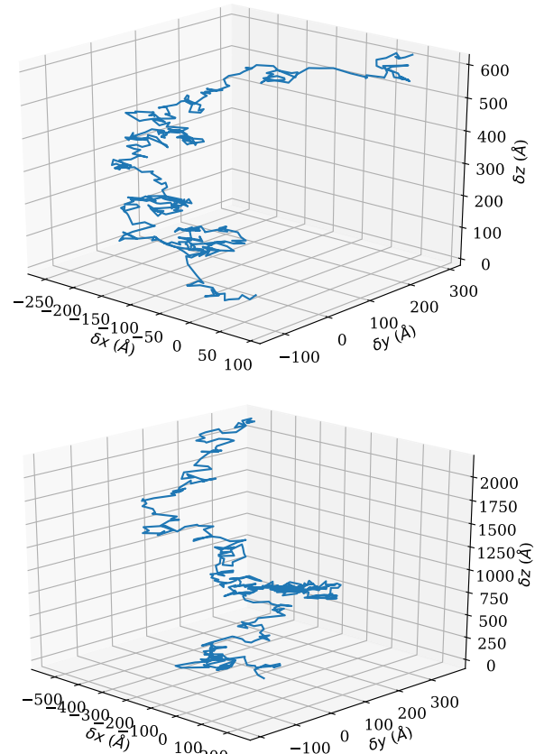
FIGURE A.1 400 000 steps trajectories of the H + species. The top (bottom) trajectory has been computed at 600 K (1 200 K). For clarity, coordinates have been printed each 1 000 steps.
