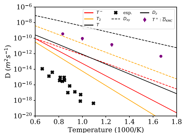
FIGURE 10 (Color online) Diffusion coefficients of T^+ , T^- , T_2 , and T in the BeO bulk compared to the experimental data of tritium diffusion in single BeO crystal. 12
