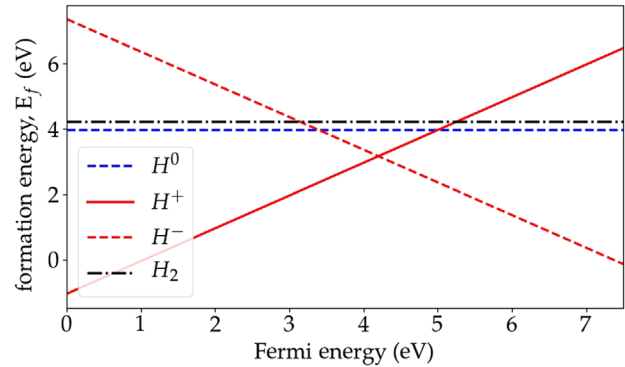
FIGURE C.1 (Color online) Formation energies of interstitial hydrogen in BeO as function of Fermi level, calculated with PBE. Only the most stable site for each hydrogen form was considered. The origin of Fermi energy is set at the top of valence band maximum. PBE, Perdew–Burke–Ernzerhof.
