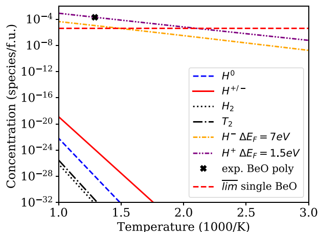
FIGURE 5 (Color online) Solubility of hydrogen (atom or molecule) as a function of its charge state. The constraint [H^+] = [H^-] enforces the Fermi level for the charged species. Concentration of charged hydrogen atom for two Fermi levels are also shown. The experimental data related to poly-crystal sample come from Ref. [13], whereas the upper experimental solubility of the single crystal is invoked in Ref. [5]. To show the isotopic effect, only species may have the highest impact is plotted, that is, T_2 .
