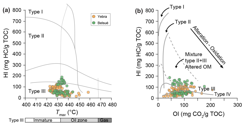
Figure 8. (a) The scatter plot of hydrogen index (HI) vs. T_{max} values allows one to discriminate between the different kerogen types, (B), whereas the scatter plot of hydrogen (HI) vs. oxygen index (OI) allows one to assess the OM source and thermal maturity. Here we display the kerogen types (a) and the OM origin (b) from Yebra de Basa (orange) and Belsué (green). Samples with TOC values lower than 0.2 wt % have been excluded. Reference lines for kerogen types and maturity after Espitalié (1986).
