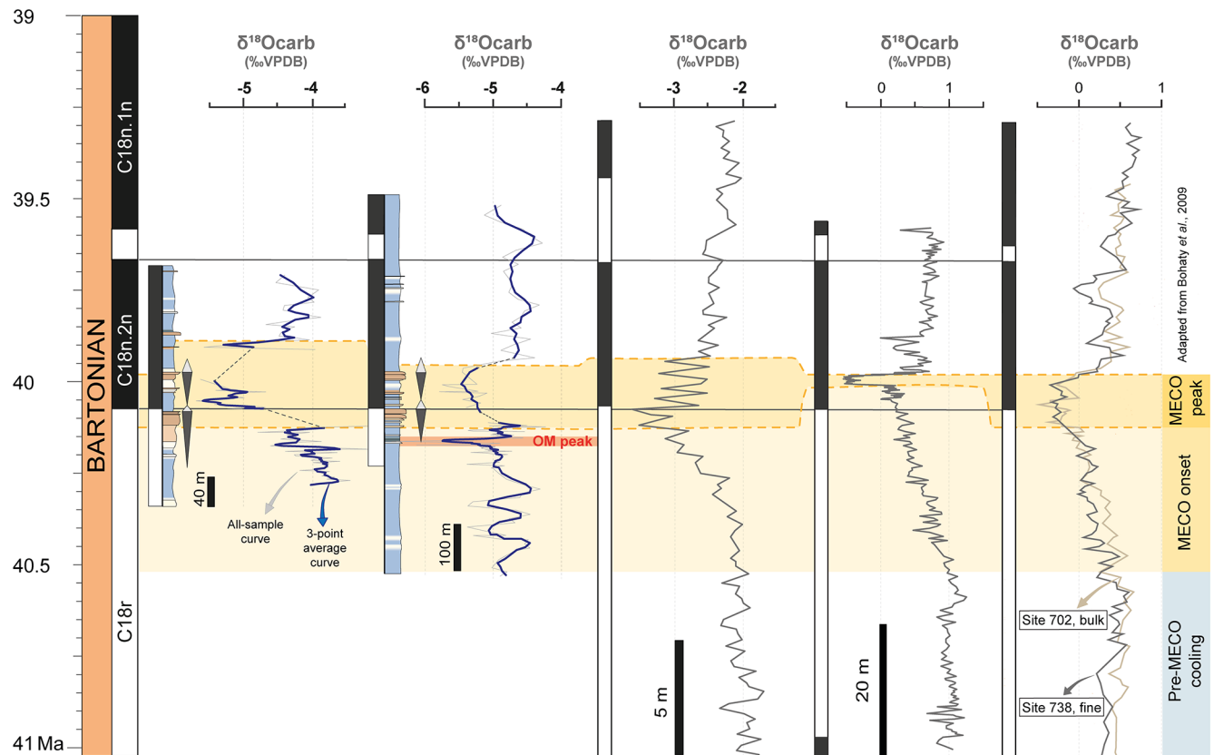
Figure 9. Oxygen isotope ( \delta^{18}\text{O}_{\text{carb}} ) correlation panel for the studied sections (Belsué and Yebra de Basa) with MECO target curves from Alano (Italy, Tethys Ocean; Spofforth et al., 2010), ODPS 1051 (N Atlantic Ocean; Edgar et al., 2010), ODPS 702 (S Atlantic Ocean; Bohaty et al., 2009), and ODPS 738 (S Indic Ocean; Bohaty et al., 2009). Data from the bulk- and fine-sediments fractions. Highlighted in red is the OM-rich interval (TOC peak) in Yebra de Basa. The two progradation–retrogradation cycles referred to in the text are drawn with grey and white triangles. The data are scaled according to magnetostratigraphic tie points, between C18r–18n.2n and C18n.2n–C18n.1n chrons.
