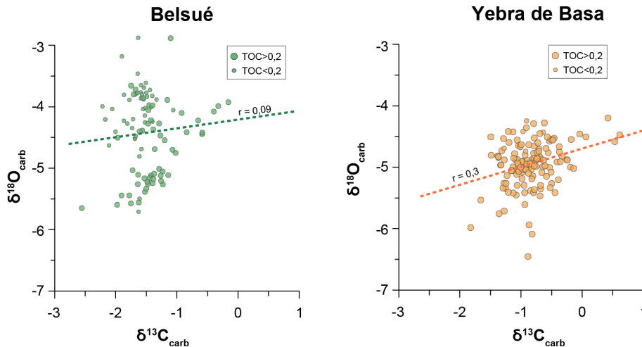
Figure 10. \delta^{18}\text{O}_{\text{carb}}-\delta^{13}\text{C}_{\text{carb}} scatterplot of all Belsué and Yebra de Basa samples. The size of the symbols is small for samples with TOC < 0.2 wt % and big for samples with TOC > 0.2 wt %. The Pearson correlation coefficients ( r ) and regression lines are shown.
