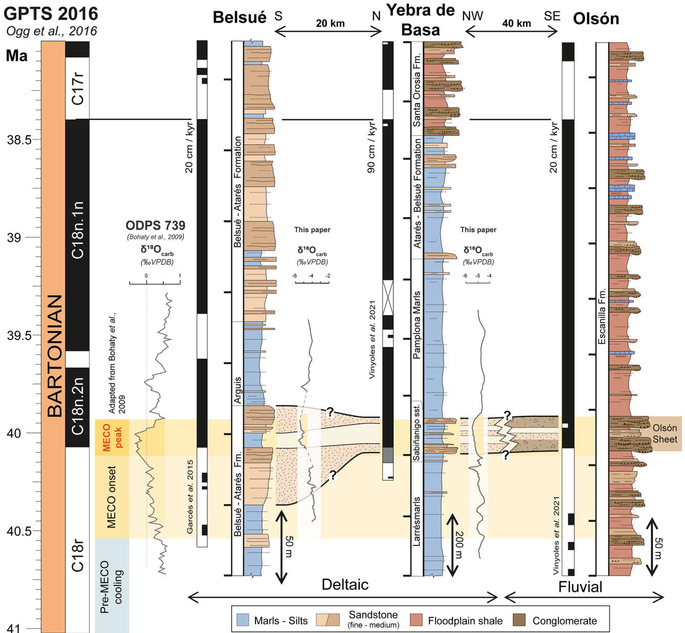
Figure 11. Correlation panel between Belsué, Yebra de Basa, and Olsón section with the GPTS 2016 (Ogg et al., 2016). The stratigraphic sections are modified from Garcés et al. (2014) and Vinyoles et al. (2021). The oxygen isotopic ( \delta^{18}\text{O}_{\text{carb}} ) record from ODPS 738 and the MECO age constraints defined by yellow and blue bars are modified from Bohaty et al. (2009). The oxygen isotopic record ( \delta^{18}\text{O}_{\text{carb}} ) from Belsué and Yebra de Basa corresponds to our results, and the dashed lines represent non-sample intervals. The sedimentation rates (SRs) from Belsué, Yebra de Basa, and Olsón are the average SR between chron C18n.2n and C17r, as from the data of Vinyoles et al. (2021).
