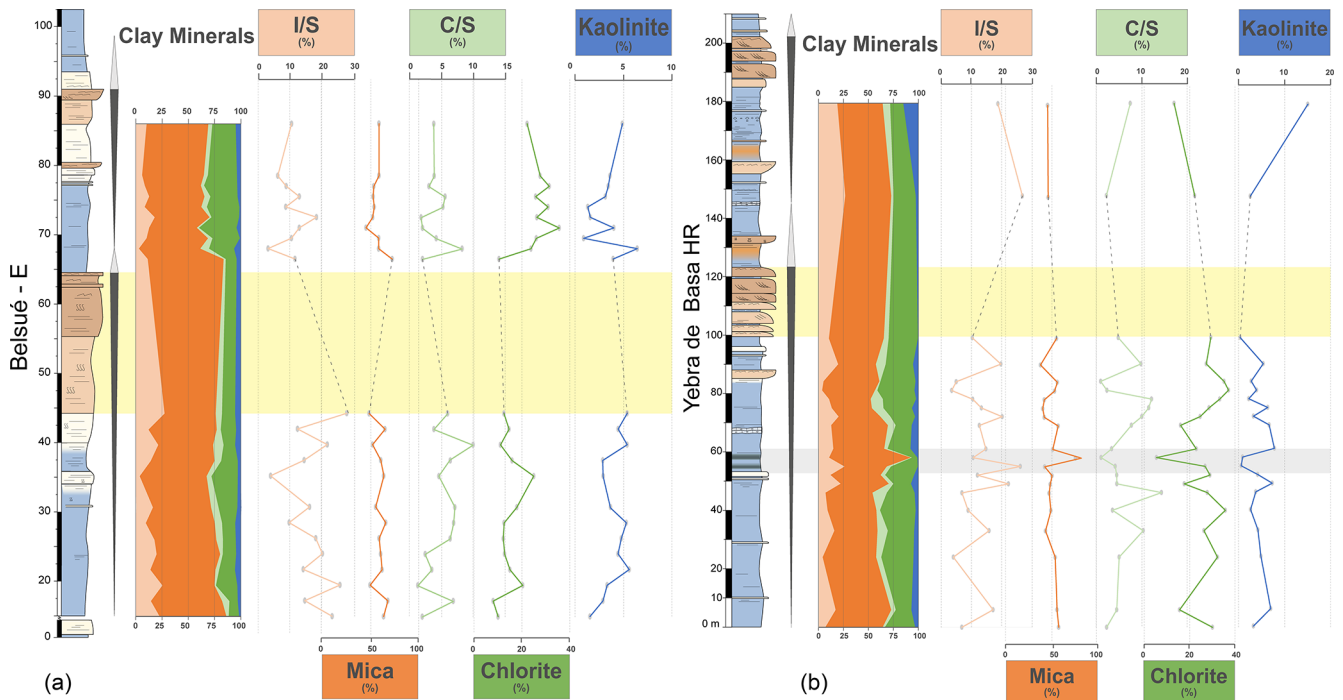
Figure 5. Schematic stratigraphic log of Belsué – E (a) and Yebra de Basa HR (b) with clay mineral assemblages, IS (illite–smectite), CS (chlorite–smectite), mica, chlorite, and kaolinite. Highlighted in pale grey is the OM-rich interval in Yebra de Basa, and in pale yellow are the main sandstone levels. The progradation–retrogradation cycles (P–R) are drawn with grey and white triangles. The dashed lines represent non-sampled intervals.
