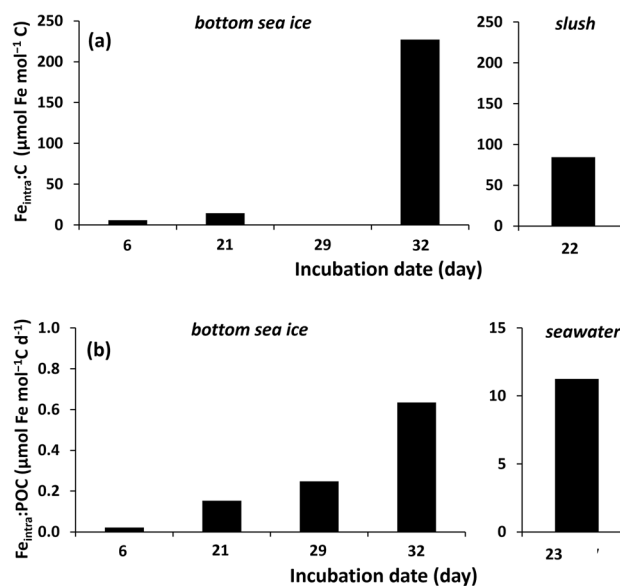
Fig. 7 Ratios of a Fe_{intra} uptake to ^{14}C uptake and b Fe_{intra} uptake to POC concentration. The uptake ratios in a do not include values for bottom sea ice on Day 29 or under-ice seawater on Day 23 due to extremely low values for ^{14}C uptake measured in those samples (Fig. 6). Ratios of Fe_{intra} uptake to POC concentration in b do not include a ratio for slush because POC in slush was not measured
