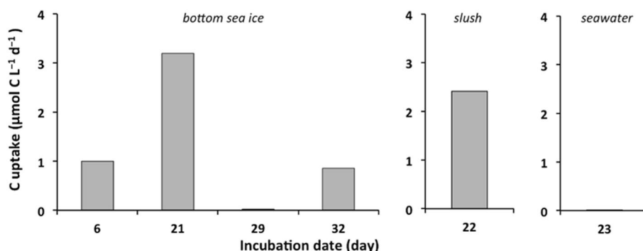
Fig. 6 ^{14}C uptake rates in bottom sea-ice, slush, and under-ice seawater samples. Short-term ^{14}C incubations were performed on 1-cm-thick bottom sea-ice sections under temperature-controlled laboratory conditions (Day 6 and Day 29) or in situ conditions (Day 21 and Day
