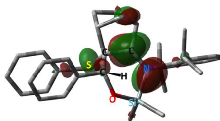
Figure 3. Optimized molecular structure of cation 2a and calculated surface diagram of its LUMO ( E = -4.24 eV, isodensity value: 0.04).
