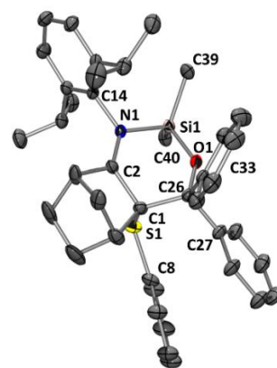
Figure 2. Molecular structure of cationic part of imine-stabilized silylium borate 2e . Thermal ellipsoids represent 30 % probability. H and disordered atoms, counterion [\text{B}(\text{C}_6\text{F}_5)_4^-] and solvent molecule were omitted for clarity. Selected bond lengths [Å] and angles [ ^\circ ]: N1-Si1 1.839(3), Si1-O1 1.614(3), C26-O1 1.428(5), S1-C1 1.857(4), C1-C2 1.550(6), C2-N1 1.292(5), N1-C14 1.484(5), S1-C8 1.804(4), C26-C33 1.542(6), C26-C27 1.559(9), Si1-C39 1.823(4), Si1-C40 1.838(4); N1-Si1-O1 99.8(1), Si1-O1-C26 135.4(2), C26-C1-C2 111.6(3), C1-C2-N1 124.3(4), C2-N1-Si1 120.0(3), O1-C26-C1 105.8(3), C2-N1-C14 120.9(3), C14-N1-Si1 118.8(2), O1-Si1-C39 111.8(2), O1-Si1-C40 112.4(2).
