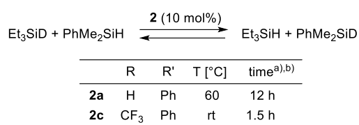
Figure 4. H/D exchange between Et 3 SiD and PhMe 2 SiH catalyzed by 2 . a) Time to achieve the 38 : 62 ratio of Et 3 SiD/Et 3 SiH. b) Determined by 1 H-NMR monitoring of PhMe 2 SiH/Et 3 SiH.
