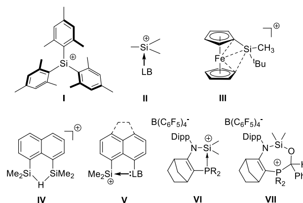
Figure 1. Free silylium ion I and Lewis base-stabilized silylium ions II-VII .
