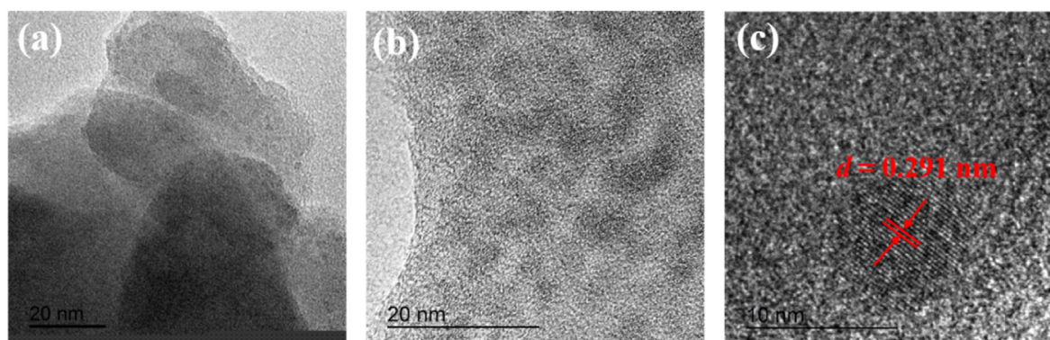
Fig. 1. Transmission electron microscopy (TEM) images of the NZ (a) and NZA (b) samples and high-resolution (HR)TEM image of NZA sample (c).
