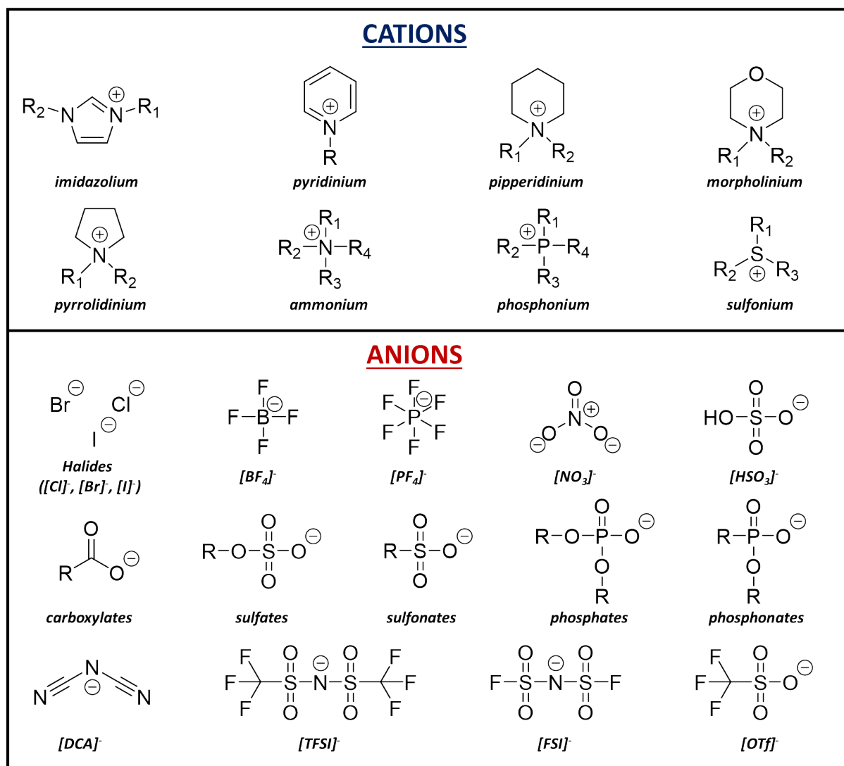
Figure 3. Common cations and anions of ILs. R represents the typical substitution sites, R = H or alkyl.
