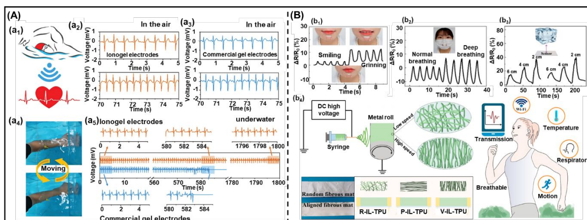
Figure 10. (A) Schematic illustration biocompatible PVA-tannic acid-cholinium lactate (PVA-TA-[Ch] + [Lac] - ) ionogel for ECG recording in the air and underwater. (a 1 ) Schematic diagram of ECG signal detected by ionogel electrode underwater; (a 2 ) ECG signals recorded by ionogel electrode when a volunteer is at rest (top) and running (bottom); (a 3 ) ECG signals recorded by CGE while the volunteer was resting (top) and running (bottom); (a 4 ) Photos of ECG signals detected by ionogel electrode during human movement underwater; (a 5 ) Long-term stability of ECG signal detected by CGE and ionogel electrode in the aquatic environment. Reproduced with permission from ref. 29 . Copyright 2021, John Wiley & Sons, Inc. (B) Schematic demonstration of V-IL/TPU ionogel sensor. Real-time response of the V-IL/TPU sensor to the
