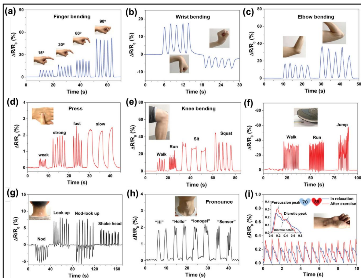
Figure 9. Real-time monitoring of human motions and subtle physiological signals by ionogel-based sensors. Signals of relative electrical resistance during a) finger bending, b) wrist bending, c) elbow bending, d) press, e) knee bending, f) walking, running, and jumping, and g) neck movements. Relative resistance variations during h) speaking different words and i) radial pulse of the wrist at ease and after exercise. Inset: variations of wrist pulse patterns with an unnoticeable tidal wave at ease (blue) and a high tidal peak after R1-exercise (red). Permission from ref. 217 Copyright 2021, John Wiley & Sons, Inc.
