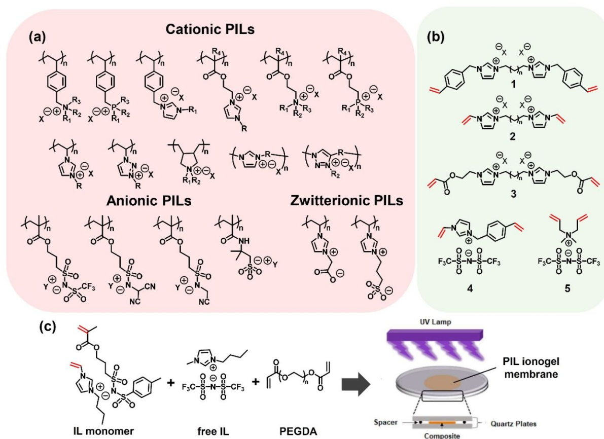
Figure 6. (a) Examples of chemical structure of cationic, anionic and zwitterionic PILs. ( R , R_1 , R_2 and R_3 = alkyl or phenyl; R_4 = H or methyl). (b) Examples of chemical structure of IL cross-linkers. (c) Illustration of PIL ionogel membrane preparation via photo-polymerization. Adapted from ref. 158 with permission from American Chemical Society, Copyright 2020.
