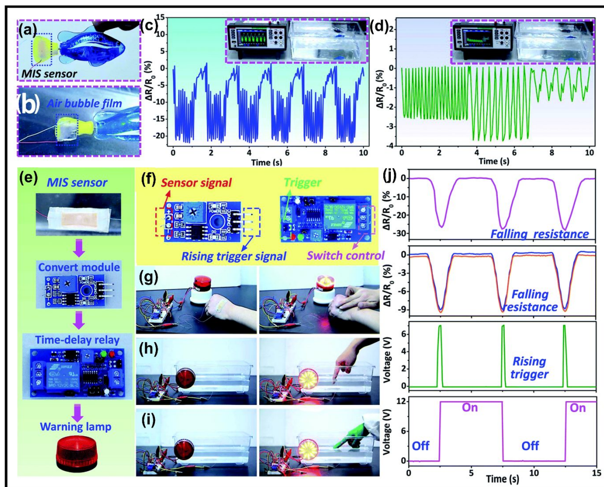
Figure 12. (a-d) Applications of the MIS-based sensors in real-time detection of motions and subtle vibrations in an aqueous environment. (a) MIS sensor attached to the robotic “fishtail”, (b) a layer of significant air bubble film forms on the MIS sensor due to its excellent superhydrophobicity. (c-d) the relative resistance variations of the MIS sensor in response to the constant and different swing frequencies of the “fishtail”. (e–j) Applications of MIS sensor in a smart warning lamp control system. (e) Photographs of the circuit of the alarm lamp control system. (f) The functions performed by the conversion module and the time delay relay during signal transmission. (g–i) Application of the alarm lamp control system in different scenarios. (j) the corresponding signal transmission and conversion process. Permission from ref. 270 . Copyright 2021, Royal Society of Chemistry.
