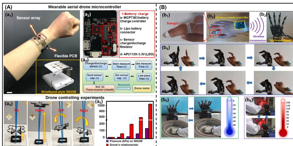
Figure 11. (A) (a 1 ) Photograph of a WADM (fabricated by integrating the IL–silica–TPU flexible pressure sensor array of 4 pixels and flexible wireless PCB) attached to a wrist. Scale bar, 2 cm. (a 2 ) Photograph of commercially available flexible wireless PCB with different integrated circuit components labeling. (a 3 ) System-level functional block diagram of WADM shows different steps of signal processing and wireless transmission features enabling aerial drone control. (a 4 ) Photographs of real-time experiments of aerial drone control, which include
