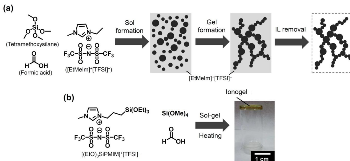
Figure 5. Examples of ionogel preparation through sol-gel reactions. (a) Scheme of sol-gel processes. Reproduced with permission from ref 146 . Copyright 2000, Royal Society of Chemistry. (b) Molecular structures of gel precursors and [(\text{EtO})_3\text{SiPMIM}]^+[\text{TFSI}]^- ionic liquid and the image of the obtained ionogel. Reproduced with permission from ref 149 . Copyright 2014, Royal Society of Chemistry.
