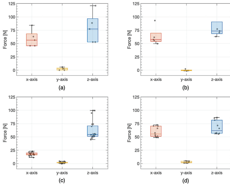
Fig. 29 Summary of the force load cell measurements along the x-, y-, and z-directions for (a) a push with the flat part of the scoop near where the HP 3 was deployed, (b) a push with the scoop tip near the mole hole, (c) a push with the bottom of the scoop where the indentation and first elastic properties experiments were performed, and (d) a push with the bottom of the scoop where the second elastic properties experiment was performed. Grey dots represent individual data points. Box and whisker plots represent the data distribution for F_x , F_y , and F_z . For each box, the central horizontal line indicates the median, and the bottom and top edges of the box indicate the 25th and 75th percentiles, respectively. The whiskers extend to the most extreme data points not including outliers
