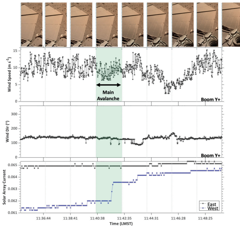
Fig. 23 Progressive IDC images of northwestern edge of the lander and the southeastern edge of the western solar array during the arm motion and dump of soil along with wind speed and direction from the TWINS +Y sensor and the detrended solar array current on both panels. The main avalanche from the scoop occurred between 11:40 and 11:42 LMST on sol 884 and resulted in a 3% increase in solar array current for the west array
