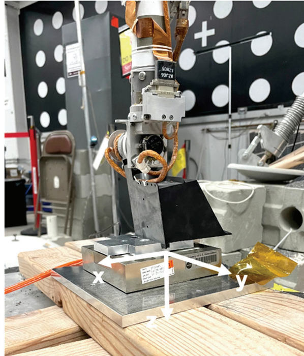
Fig. 28 Picture of the IDA scoop and multi-axis load cell in the testbed. Flat bottom of the IDA scoop is pressing on the multi-axis load cell setup at the Indentation and Elastic Properties location. Directions of the x-, y-, and z-axis forces are shown. Note the scoop tip to the right and the secondary blade on the bottom left. Note portion of calibration target (white circles on black background) against the wall behind the lander and the lander footpad to the right
