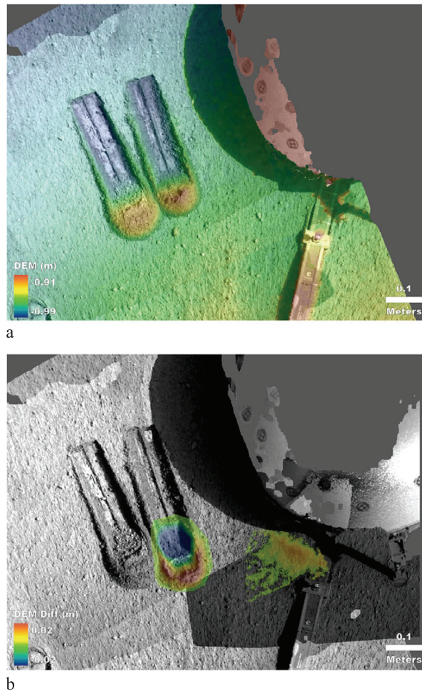
Fig. 10 DEMs showing how volumes of scoops and piles were determined. a) IDC DEM produced from stereo pair after scrapes on sols 802 and 803. Note ridges of material on the sides and bulldozed piles at the ends of the scrapes. The slopes of the bulldozed soil piles are between 42^\circ \pm 2.7^\circ whereas the slopes of the walls created by the vertical sides of the scoop are between 54.7^\circ \pm 6.6^\circ . b) IDC differenced DEM from sol 816 (after the scoop) minus sol 803 (before the scoop) showing differences where the scoop removed soil (left) and where soil was added in a pile after the dump (right). The differenced volume of the scoop trough ( -214.4 \text{ cm}^3 ) minus the scoop ridge ( 121.5 \text{ cm}^3 ) yields a scoop volume of 92.9 \pm 8.4 \text{ cm}^3 . The increase in volume of the pile on the tether is 61.7 \pm 12.3 \text{ cm}^3 . The difference between the volume of the soil in the scoop and the volume of soil in the pile is 31.2 \pm 20.7 \text{ cm}^3 , which is an estimate of the volume of material dispersed by the wind ( \sim 31\% of the scoop). The slope of the pile on the tether is 24.1^\circ \pm 6.1^\circ
