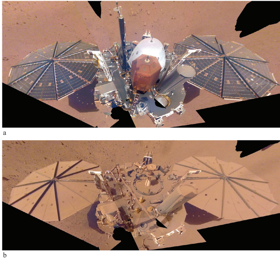
Fig. 18 Lander selfies acquired after landing on sol 10 (a) and near the end of the mission on sol 1211 (b) showing the dust that has accumulated on the lander and solar panels over 2 Mars years on the surface. The energy from the solar panels had decreased to about 10% of that at the start by the end of the mission. Note instruments on the deck for (a) and not for (b) and the piles of soil on the northwest portion of the deck from the solar array cleaning experiments
