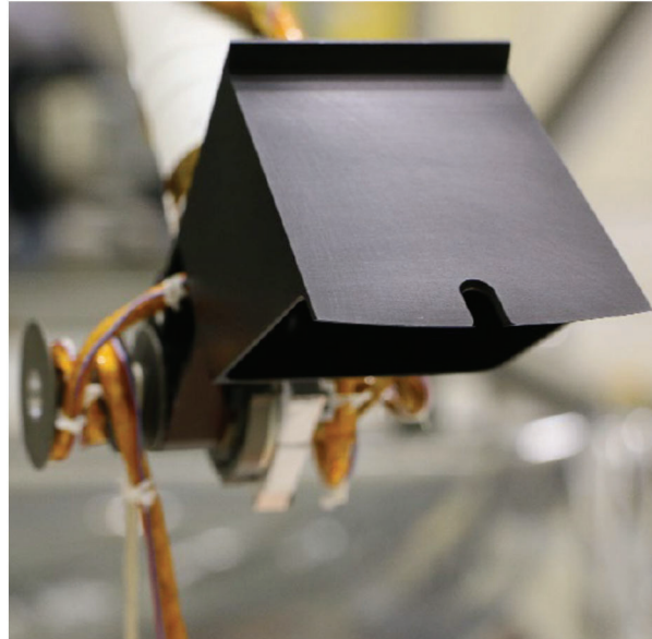
Fig. 3 The scoop at the end of the IDA. Note the blade on the tip of the scope with semicircle cut out and the second blade on the bottom. The width of the scoop is 7.5 cm and it holds a volume of 250 cm 3 . Note attachment to the wrist joint, which provides one degree of freedom motion
