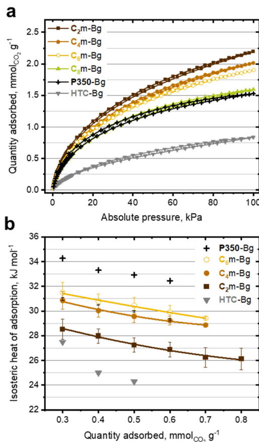
Fig. 5 (a) Carbon dioxide sorption isotherms at 273 K of C 2 m-Bg , C 4 m-Bg , C 6 m-Bg , C 8 m-Bg , P350-Bg and HTC-Bg . (b) Isosteric heat of adsorption of CO 2 for HTC-Bg , C 2 m-Bg , C 4 m-Bg , C 6 m-Bg and P350-Bg . The isosteric heat of adsorption was calculated by applying the Clausius–Clapeyron equation to CO 2 adsorption isotherms obtained at three different temperatures (273, 298 and 323 K). Note that the isosteric heats of adsorption are given as absolute values. The corresponding isosteric enthalpies of adsorption are negative.
