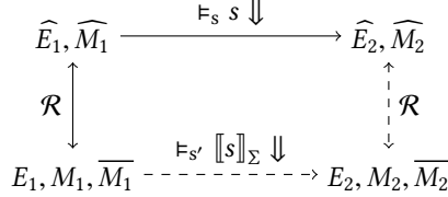
Fig. 25. Commutation diagram of the soundness theorem.
