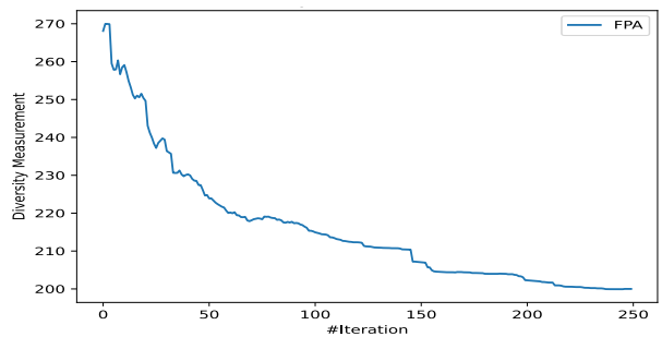
FIGURE 16. FPA diversity.
