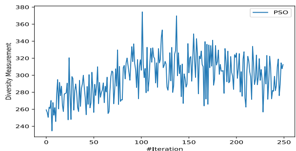
FIGURE 17. PSO diversity.
