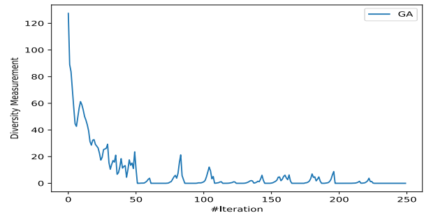
FIGURE 15. GA diversity.
