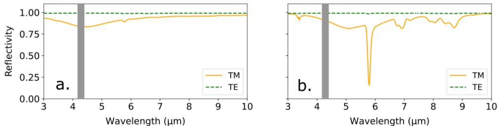
Figure 3. Measured spectra of a. the bare array and b. the array covered with a 45 nm PMMA layer, for TM (orange continuous line) and TE polarization (green dashed line). Grey areas cover the absorption of \text{CO}_2 . Dimensions h_{Au}=45 nm, h_d=280 nm, w=50 nm and d=400 nm.
