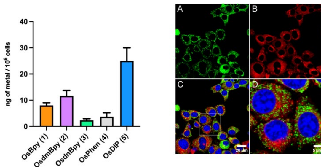
Figure 5: (Left) Cellular uptake of compounds 1–5 by ICP-MS (Right) Cellular uptake of complex 1 by confocal microscopy. A. Mitochondria-specific dye MitoTracker Green (green, exc: 488 nm, em: 513–550 nm) B. Complex 1 (red, exc: 448 nm, em: 645–730 nm) C. Overlay plus nucleus-specific dye Hoechst 33342 (blue, exc: 405 nm, em: 409–448 nm) D. Higher magnification of the boxed area in C.
