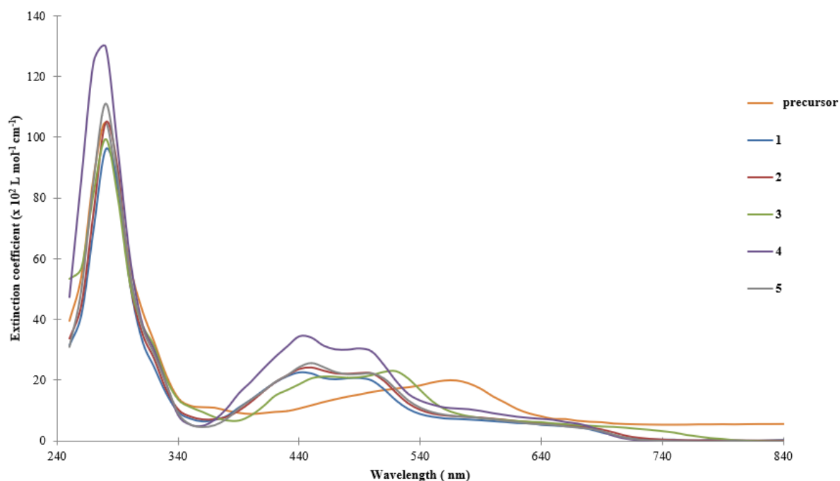
Figure 4. UV/vis/NIR spectra of complexes 1-5 and their precursor complex in CH 3 CN.
