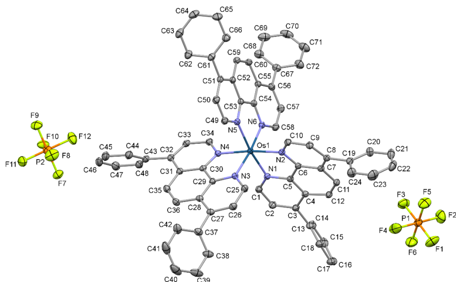
Figure 3. X-ray molecular structure of complex 5 , with hydrogen atoms omitted.
