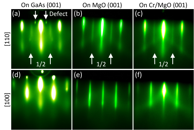
FIG. 3. RHEED images of 20-nm-thick [\text{CMA}_n/\text{FMA}_n]_q films grown on indicated substrates along Heusler (a–c) [110] and (d–f) [100] directions. Half-order streaks along [110] indicate an L2_1 -like surface unit cell. Faint spots visible in (a), which vanish after annealing to 300 °C, are attributed to crystal twinning at low growth temperatures.
