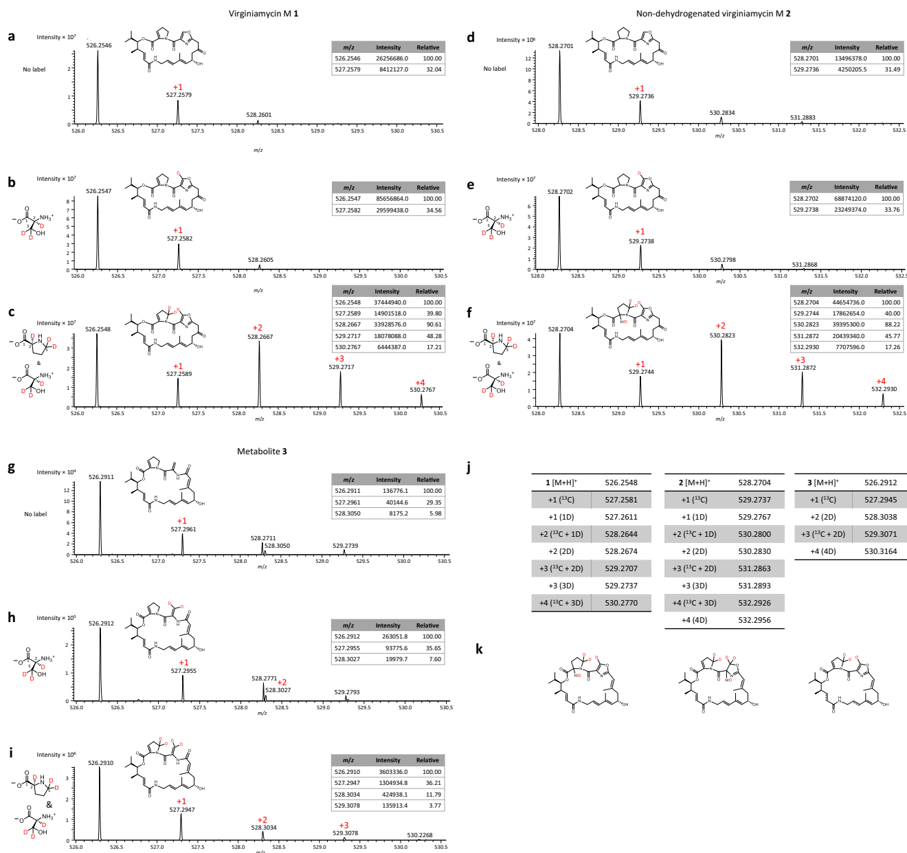
Fig. 7 | Patterns of isotope incorporation into metabolites 1–3 in the presence of labelled amino acids. a Mass spectrum of 1 ( [M + H]^+ ) obtained in the absence of feeding (the calculated masses for 1–3 are presented in Supplementary Table 5). b Mass spectrum of 1 ( [M + H]^+ ) obtained in the presence of fed L-serine-2,3,3-D 3 (the deuterated positions in the Ser and in 1 are shown in red). c Mass spectrum of 1 ( [M + H]^+ ) obtained in the presence of fed L-proline-2,5,5-D 3 and L-serine-2,3,3-D 3 . d Mass spectrum of 2 ( [M + H]^+ ) obtained in the absence of feeding. e Mass spectrum of 2 ( [M + H]^+ ) obtained in the presence of fed L-serine-2,3,3-D 3 . f Mass spectrum of 2 ( [M + H]^+ ) obtained in the presence of fed L-proline-2,5,5-D 3 and L-serine-2,3,3-D 3 . g Mass spectrum of 3 ( [M + H]^+ ) obtained in the absence of feeding. h Mass spectrum of 3 ( [M + H]^+ ) obtained in the presence of fed L-serine-2,3,3-D 3 . i Mass spectrum of 3 ( [M + H]^+ ) obtained in the presence of fed L-proline-2,5,5-D 3 and L-serine-2,3,3-D 3 . In panels a–i , the relative peak intensities are shown in inset. At the resolution at which these experiments were carried out (60 K, 200 m/z , full width at half maximum (FWHM), which translates into a resolution of 40 K at 500 m/z ), it was not possible to distinguish between two ions which have a \Delta m/z = 0.0030 AMU, which is the case with metabolites differing by the alternative presence of D (+1.0063) and 13 C (+1.0033). At 40 K, discriminating between such ions would have required a mass difference of 0.0125 AMU or greater (i.e. 4× the
