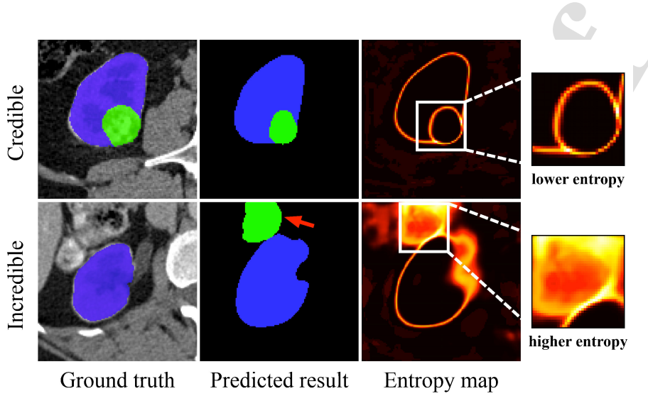
Figure 9: Different regions have different entropy, and higher entropy values generally appear along with incorrect prediction results.
