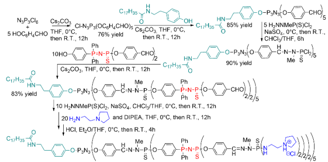
Scheme 24. Synthesis of an amphiphilic dendron bearing an alkyl chain at the core, 10 Ph 2 P=N-P=S linkages inside the structure, and 40 ammoniums on the surface.
