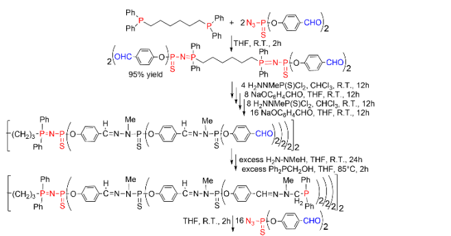
Scheme 24. Synthesis of an amphiphilic dendron bearing an alkyl chain at the core, 10 Ph 2 P=N-P=S linkages inside the structure, and 40 ammoniums on the surface.
