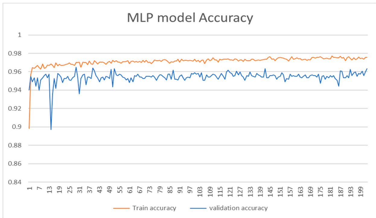
Figure 6. MLP model accuracy curve with epoch = 200.
