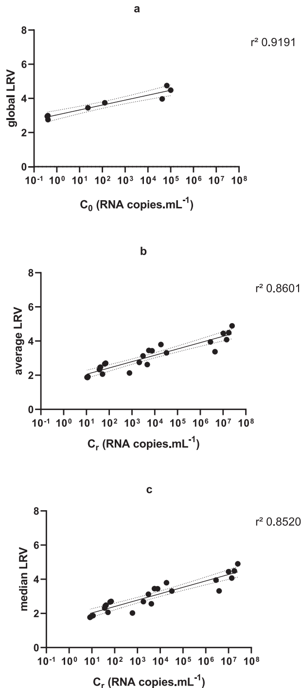
Fig. 6. Variation of global, average, median LRV as the function of the virus concentration inside the membrane [Seawater].
