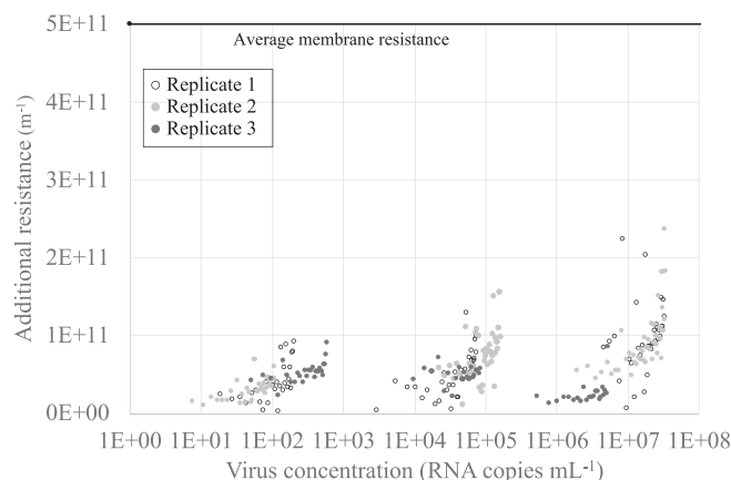
Fig. 3. Variation of the additional resistance as the function of the upstream virus concentration [Retention rate = 100%, Evian].
