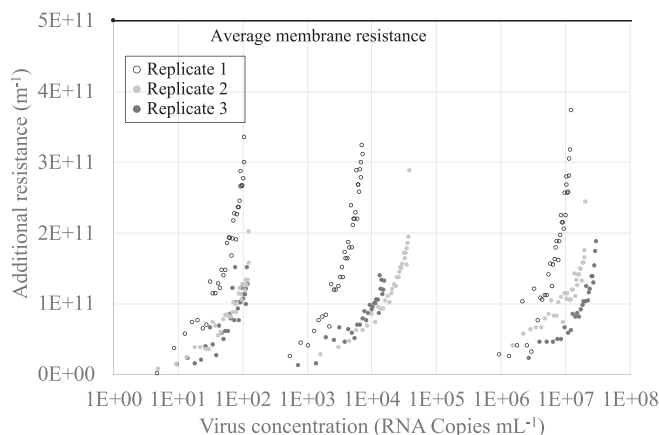
Fig. 4. Variation of the additional resistance as the function of the upstream virus concentration [Retention rate = 100%, seawater].
