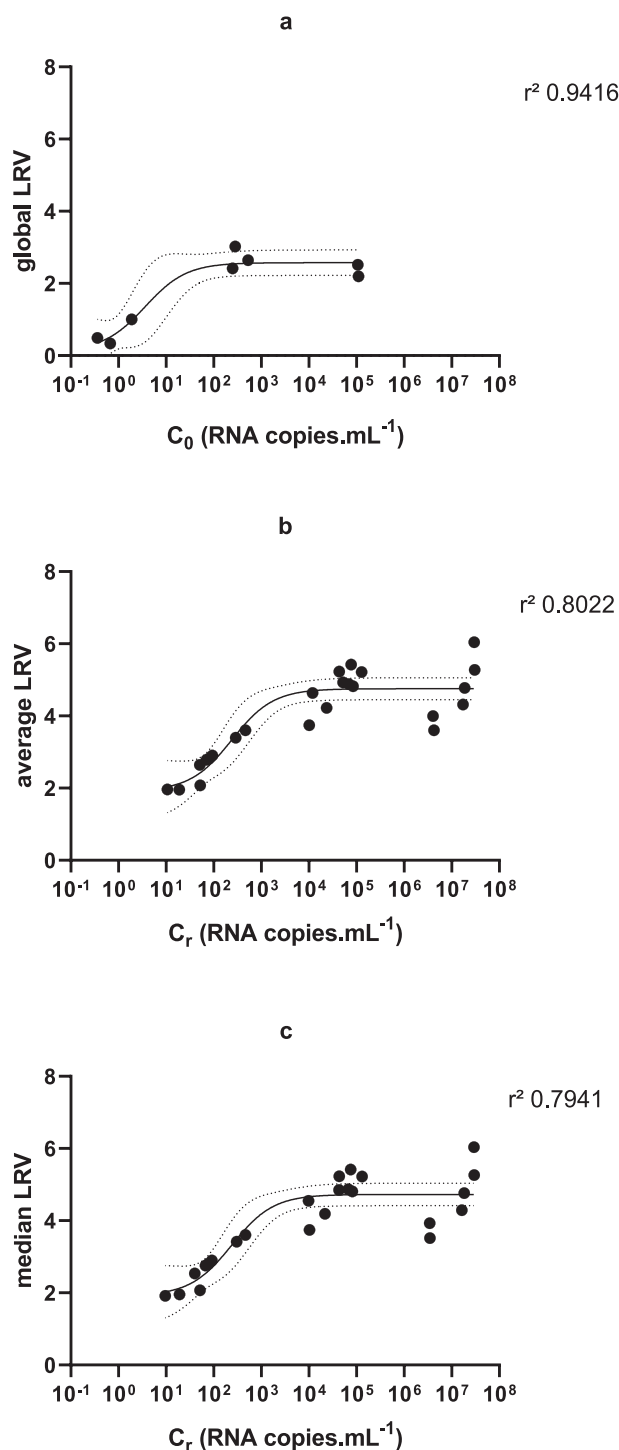
Fig. 5. Variation of global, average, median LRV as the function of the virus concentration inside the membrane [Evian].
