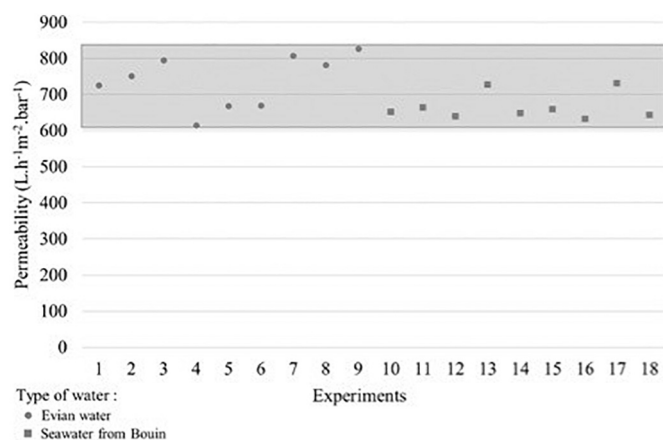
Fig. 1. Initial membrane permeabilities (with ultrapure water at 20 \text{ }^\circ\text{C} ) for all the membrane modules used
