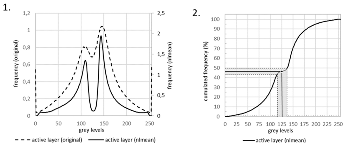
Fig. 1. Variation of (1) the grey level distribution of the original images and (2) the cumulative grey level distributions of the filtered images (active microfiltration layer).
