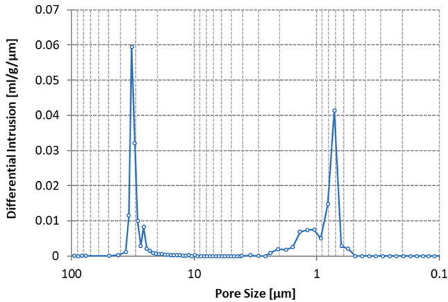
Fig. 5. Differential mercury intrusion as a function of pore size for Crystar® SiC membrane 0.6 μm.
