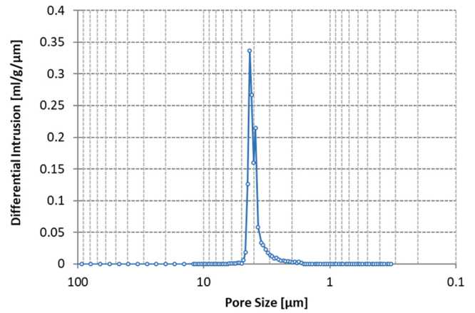
Fig. 6. Differential mercury intrusion as a function of pore size for Crystar® SiC membrane 4 μm.
