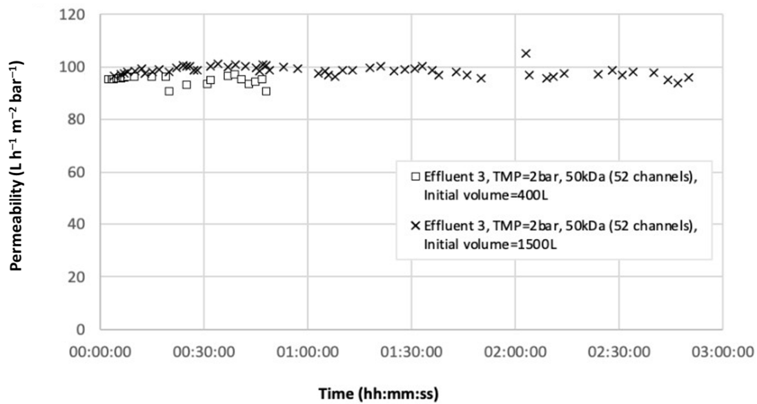
Figure 6. Permeability as a function of time.
