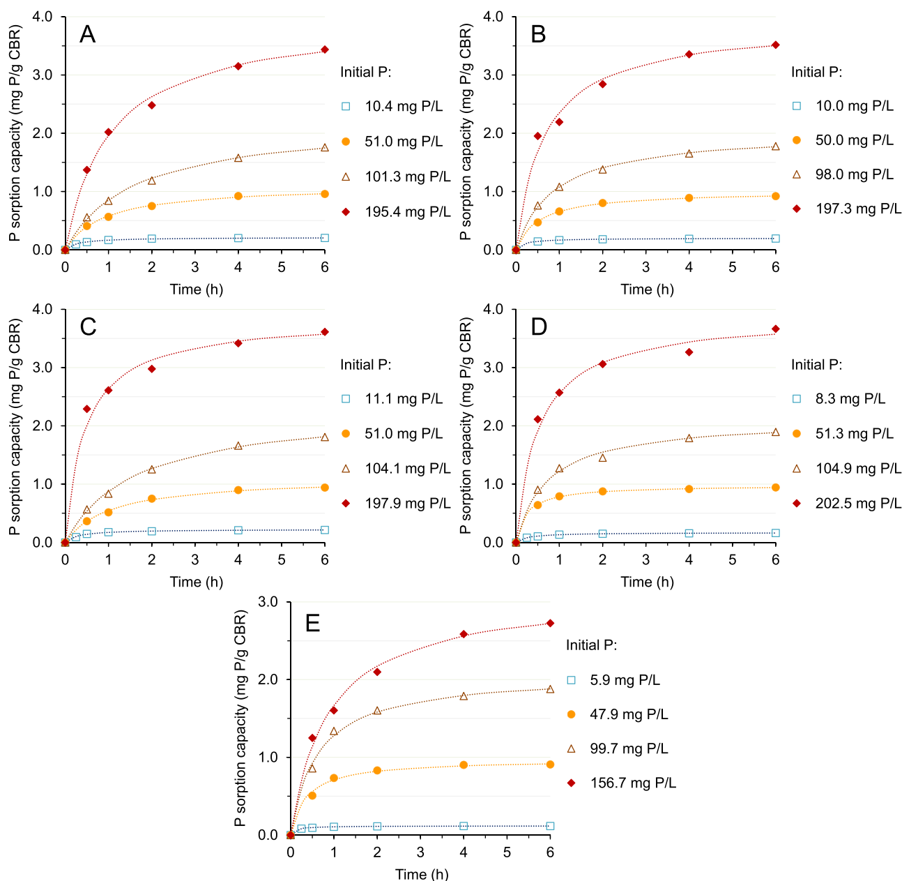
Fig. 1. Experimental P sorption capacities as a function of time for the experiments performed at different initial P concentrations and different aqueous matrices: (A) deionized water; (B) deionized water plus 40 mg N-NO 3 /L; (C) tap water; (D) tap water plus 40 mg N-NO 3 /L; (E) real effluent from a WWTP. Dotted curves show the modeled P sorption capacities using the pseudo second order kinetic equation.
