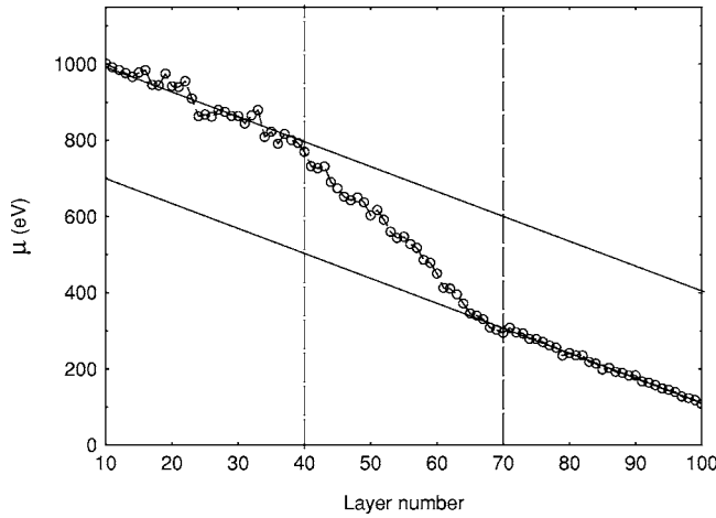
FIG. 2. The steady state chemical potential profile in a trilayer with different disorder in each layer (constant hopping matrix V = 1 eV throughout). Left to right: W/V=2 , W/V=3 , W/V=2 . The solid lines are a guide to the eye.
