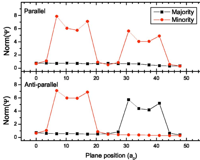
FIG. 4. (Color online.) The steady-state, norm of the wave function in each plane for parallel (P) and anti-parallel (AP) configurations ( a_0=0.529 Å).
