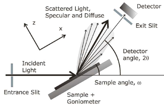
FIG. 2. (Color online) A sketch of the experimental geometry used. The x and z directions are defined with respect to the sample, and the magnetic field is applied along the x axis. The point in reciprocal space probed is determined by the settings of the sample angle \omega and the detector angle 2\theta .
