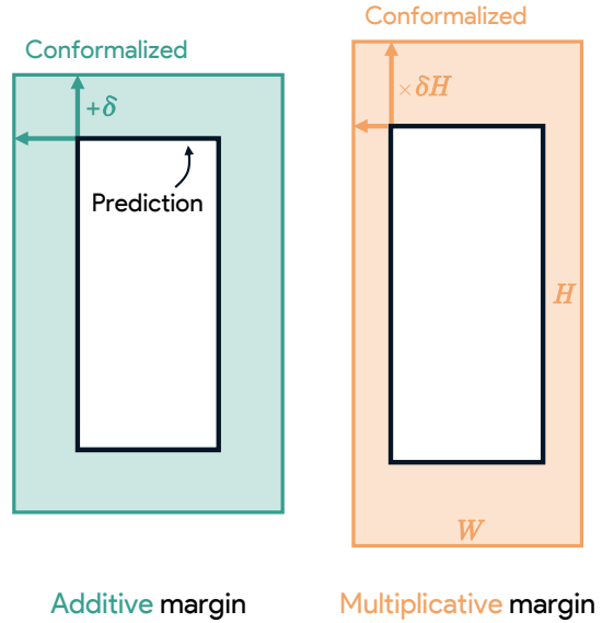
Figure 2: Effect of margin systems used.
