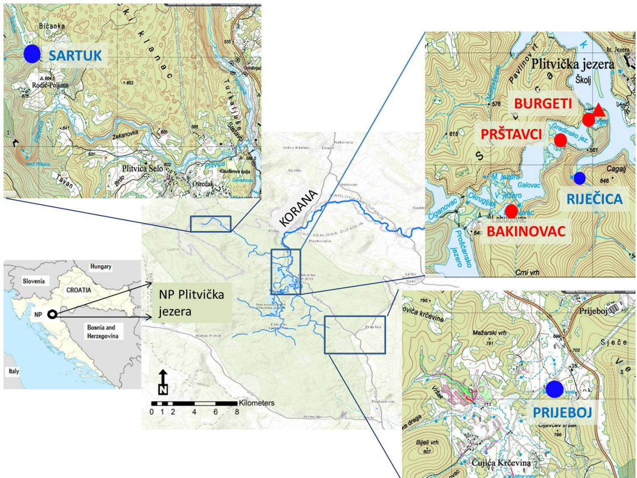
Figure 1. Position of studied sites within Plitvice Lakes National Park. Blue dots – sampled Austroptotambius torrentium populations; red dots – sampled Astacus astacus populations in 2017 and 2018; red triangle – A. astacus population sampled in 2012 and 2013. For coordinate details see Supplementary material Table S2.
