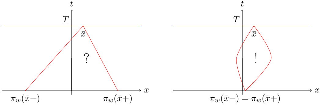
Figure 4.1: Left, in the x -independent case, extremal characteristics are straight lines and those emanating from the point of jump \bar{x} in w at time T select the segment ] \pi_w(x-), \pi_w(x+) [ along the x axis at time 0 where the initial data has no effect on w . Right, in our x -dependent choice (4.1) of the flow, characteristics bend and uniquely determine the initial data evolving into w . Note that the solution in the region delimited by the characteristics is unique.
