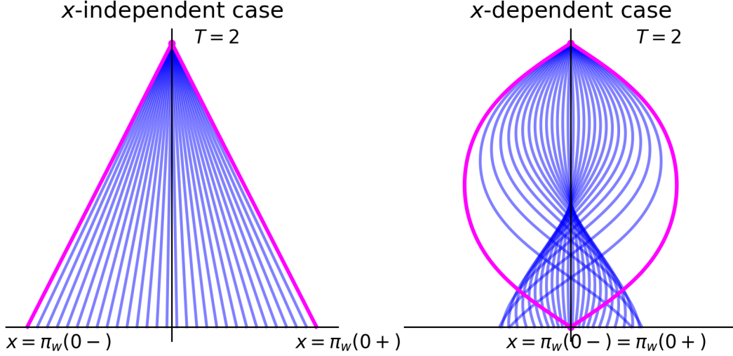
Figure 4.2: Left, in the x -independent case, the Hamiltonian rays fill the non uniqueness gap described in Figure 4.1. Right, in the x -dependent case defined by the Hamiltonian (4.1), extremal characteristics still do not intersect, but Hamiltonian rays do and may well exit the non uniqueness gap or also intersect.
