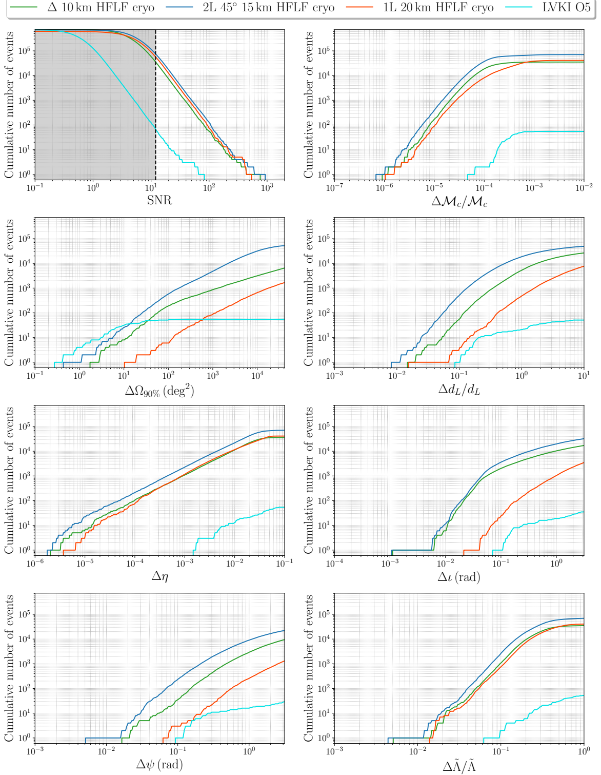
Figure 13. Comparison of SNR and parameter estimation error for a single 20 km L-shaped detector with the HFLF-cryo ASD, compared to the 10 km triangle, a 2L with 15 km arms at 45^\circ , and the forecast for LVKI O5.
