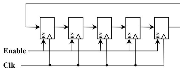
Figure 1. Token ring
