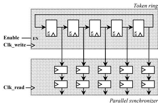
Figure 2. Synchronization of a token ring
