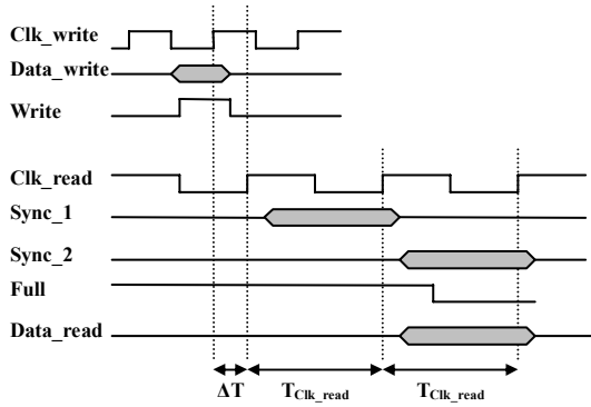
Figure 12. Latency analysis
