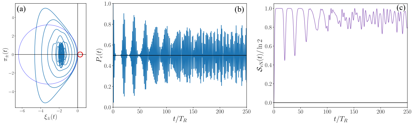
FIG. 12. Typical behavior in the metastability regime for temperature T = 0 \mu\text{K} and parameters described in the main text. (a) \xi_{\pm} phase space trajectories. (b) Rabi oscillations signal P_{eg}(t) . (c) Entanglement entropy \mathcal{S}_{\text{VN}}(t) .
