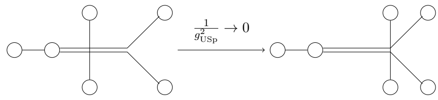
Figure 5. Brane webs for various choices of gauge coupling for the low energy theory (4.1).
