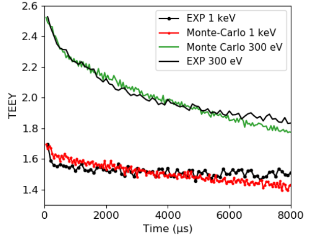
Figure 5: Comparison of the simulated and experimental data of the decrease of the TEEY
