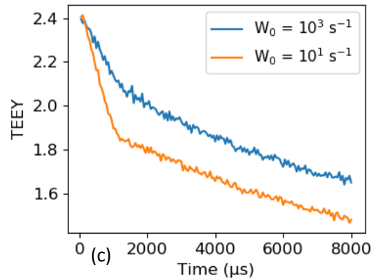
Figure 8: Effect of the model parameters on the TEEY of 500 eV electrons. (a): Effect of the capture cross sections of secondary electrons by free traps. (b): Effect of the recombination cross section. (c): effect of the detrapping frequency factor
