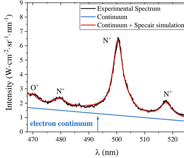
Figure 5 Fit of the N^+ and O^+ emission near the cathode at t = 9.75 ns. The continuum emission is approximated by a linear function (in blue) and the N^+ and O^+ emission is calculated by Specair (in red). The N^+ and O^+ lines are calculated, accounting for self-absorption.
