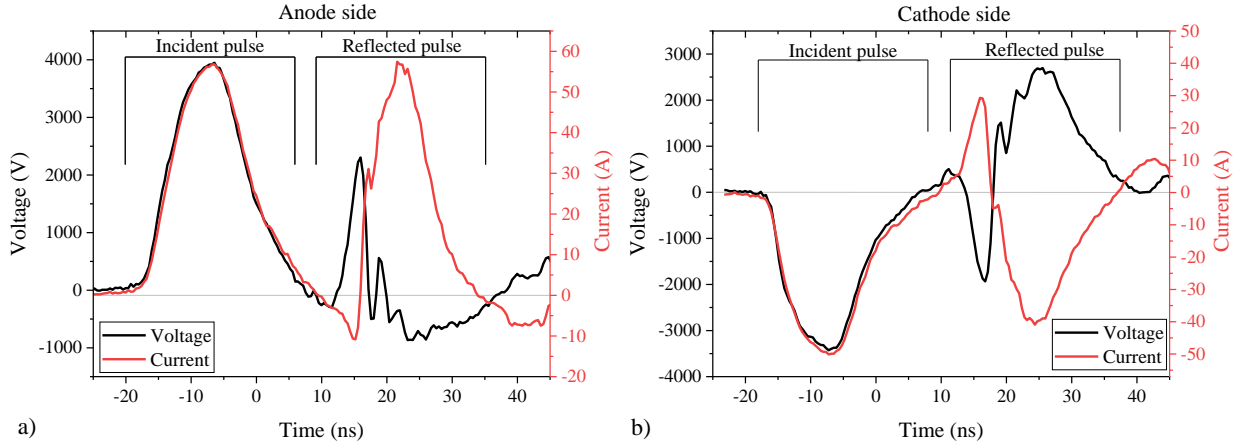
Figure 2 Measured voltage and current on a) the anode and b) the cathode sides. The amplitude difference between the incident pulses at the anode and the cathode is only due to a technical peculiarity of the pulser.
