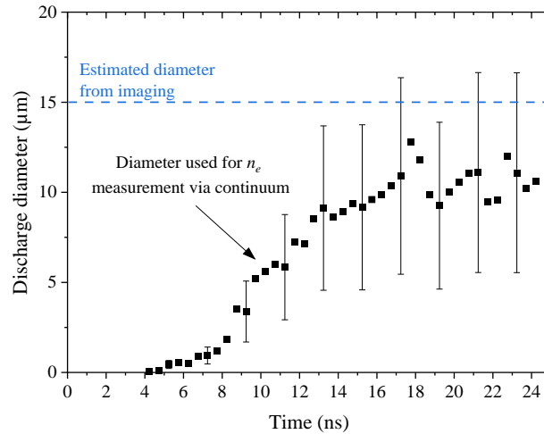
Figure 6 Discharge optical diameter evolution deduced from the ionic line radiation, and comparison with the diameter estimated using CCD imaging (dashed blue line).
