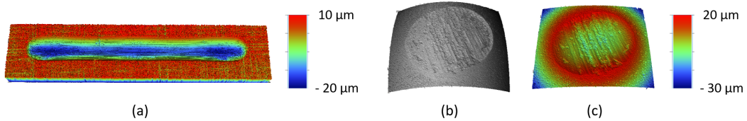
Figure 9: Optical profilometry measurements of the wear marks of the ground MAO coating (a), topography of the ball with intensity overlay (b) and ball after a sphere removal (c) measured after friction test on ground MAO coating after friction test. The deepest areas are in dark blue on the images while the highest areas are in red.
