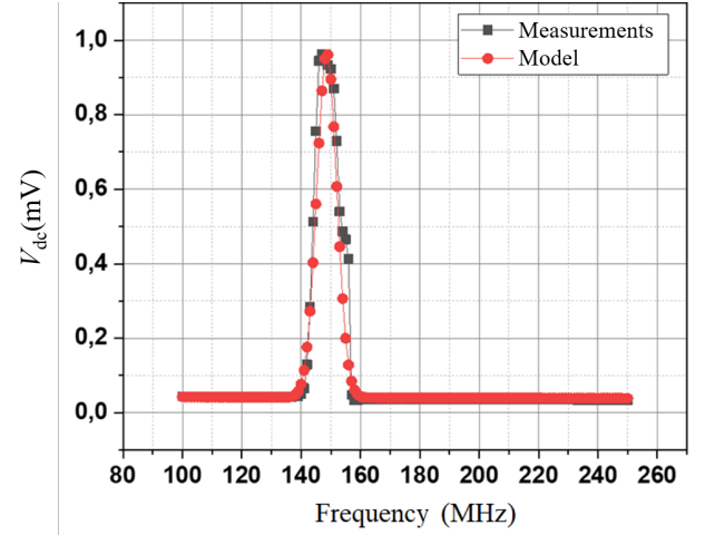
Fig. 16: CW characterization of STD_a and STD_b in series.
