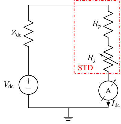
Fig. 4: DC characterization set-up for STD device.
