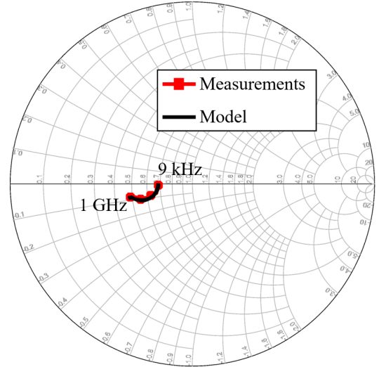
Fig. 8: Measured and simulated S_{11} reflection coefficient of the STD circuit in the frequency range [9 kHz - 1 GHz].
