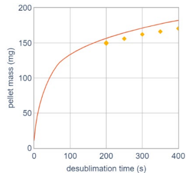
Figure 6: Model (solid line) and measurements (diamonds) comparison for 10 mm H_2 pellets, cold zone at 5 K and desub. pres. at 12 mbar.
