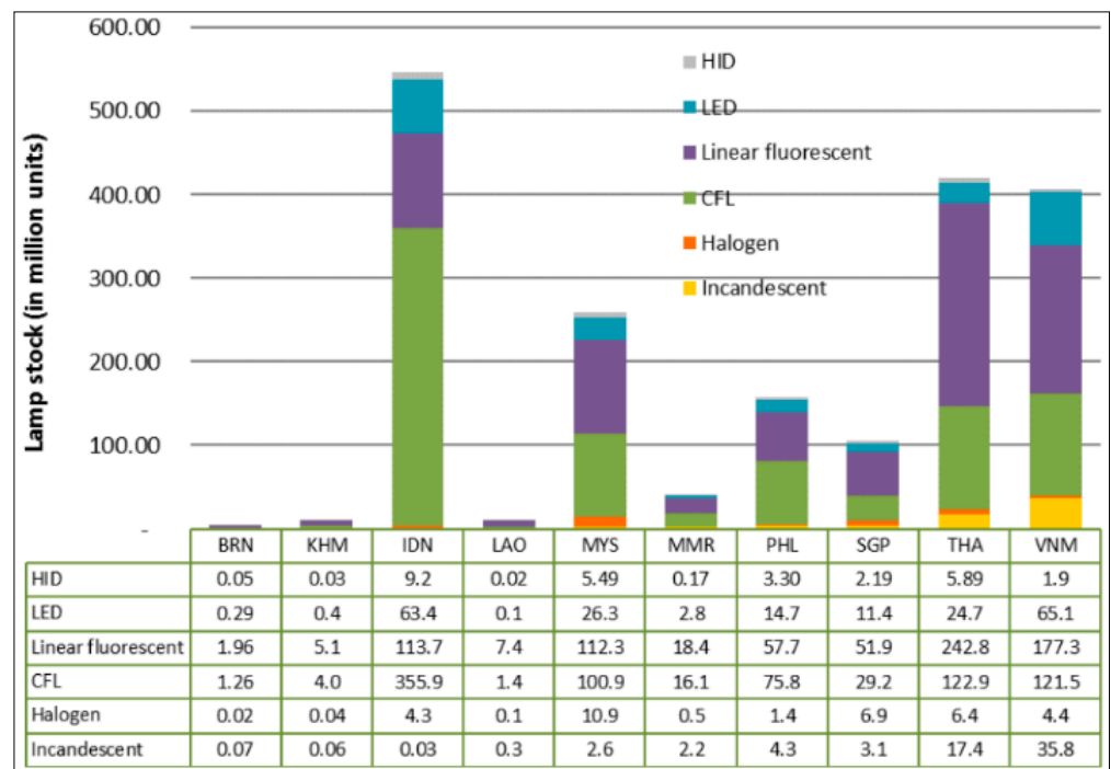
Figure 33. Lighting stock estimation in ASEAN 2014 [26].
