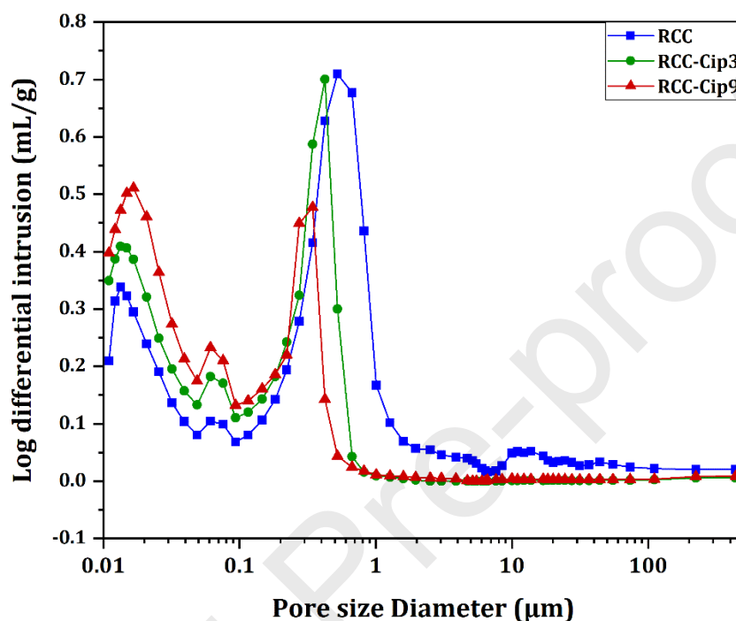
Figure 4. Pore size distribution of reference cement (RCC) and cements filled with 3% and 9% Cip (RCC-Cip3 and (RCC-Cip9).
