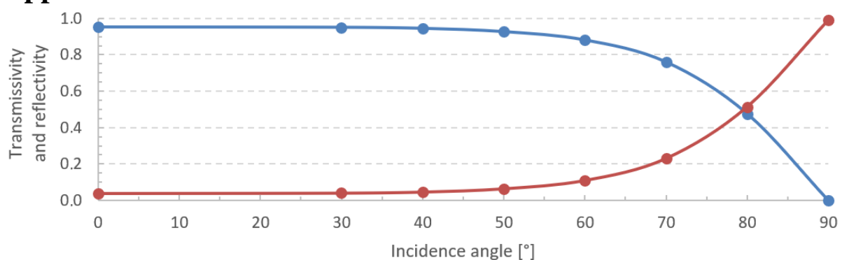
Figure A.1: Angle-dependent optical properties of the glass cover
