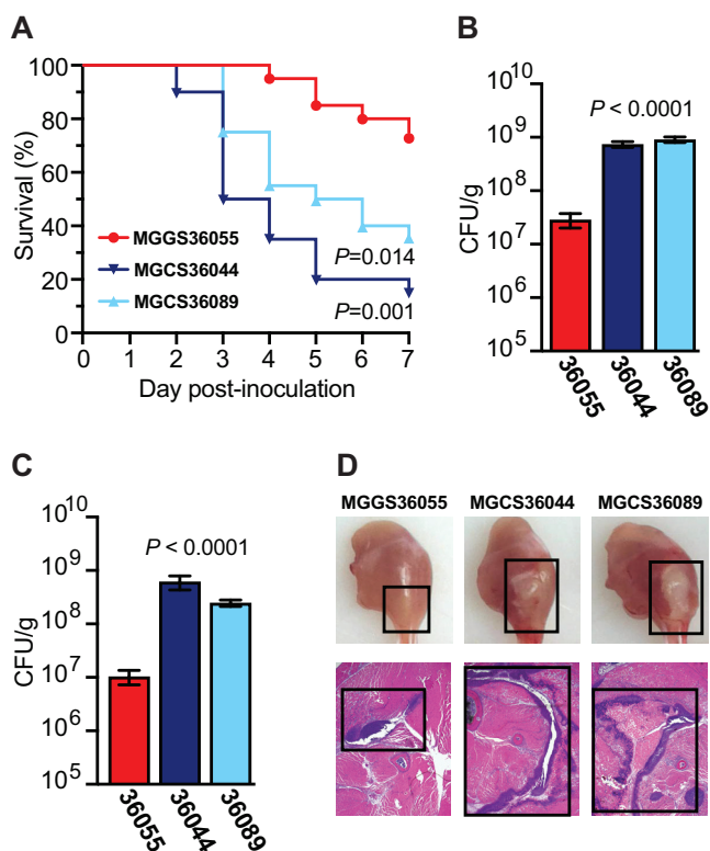
FIG 5 Virulence assessment of emm type stG62647 strains MGCS36044 and MGCS36089 and stC74a strain MGGS36055 in a mouse model of necrotizing myositis. (A) Kaplan-Meier survival curves are shown. Survival was monitored for 7 days (log-rank test, n = 20 mice per strain). (B and C) CFU recovery from infected limbs was performed on day 1 and day 2 after infection. Replicate data are expressed as means \pm SEM (Kruskal-Wallis test, n = 20 mice per strain). (D) Gross and microscopic examination of infected limbs on day 2 postinfection. Lesion size and necrotic tissue are highlighted (black boxes).
