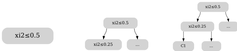
(e) Taking an IGA in the IBMPD adds a decision node to a DT.
