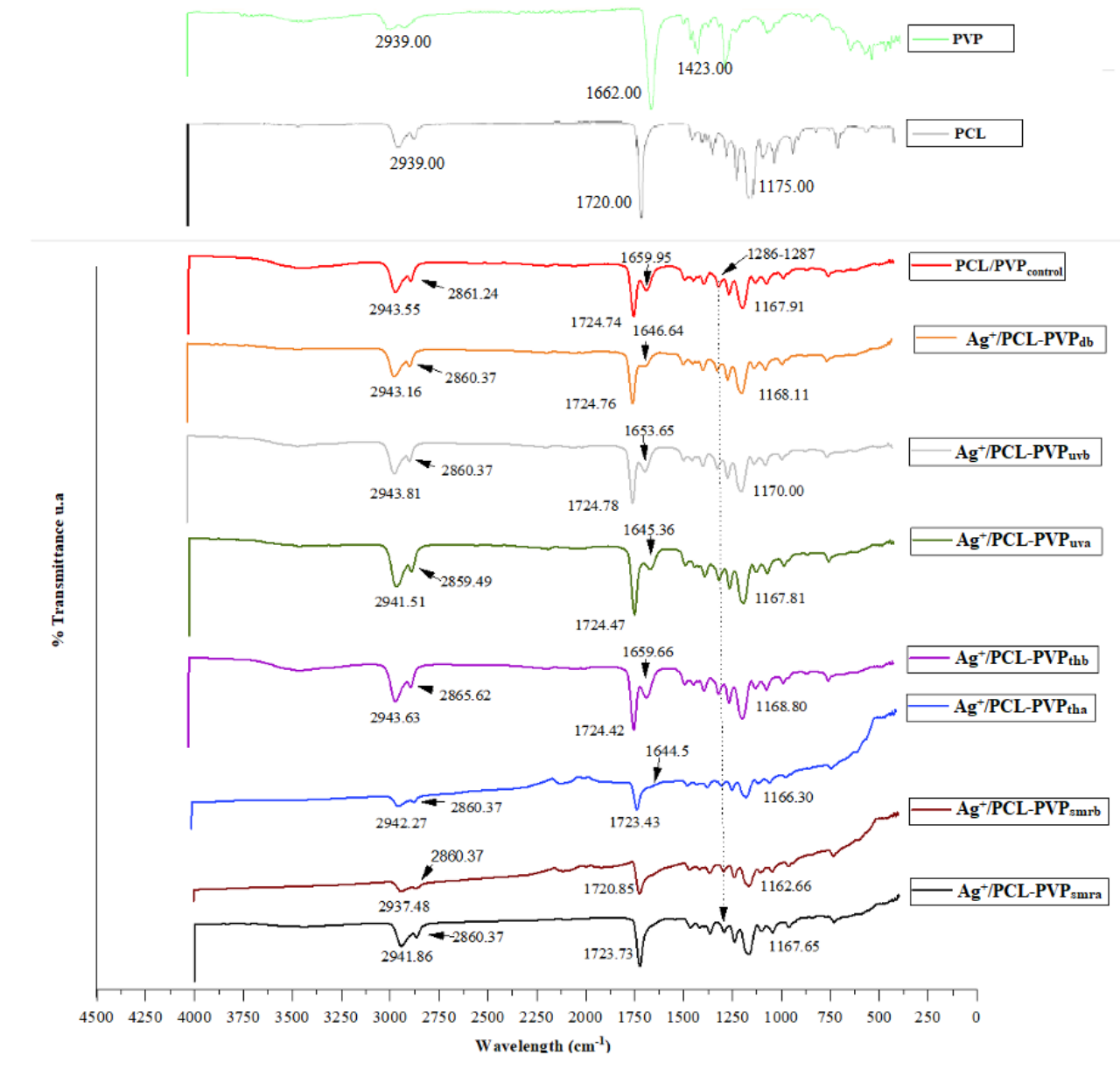
Figure 6. FTIR spectra of PCL-PVP and \text{Ag}^+ /PCL-PVP scaffolds. The black arrow indicates the presence of a 1286\text{--}1287\text{ cm}^{-1} signal in the spectra of all samples. The addition of \text{AgNO}_3 , either in the mixture or as a post-electrospinning treatment, did not affect the molecular composition of the PCL-PVP polymer.
