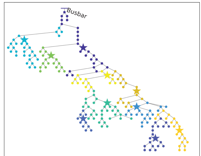
FIGURE 7 Clusters (colours) and the 10 fault positions tested (pentagram nodes)
