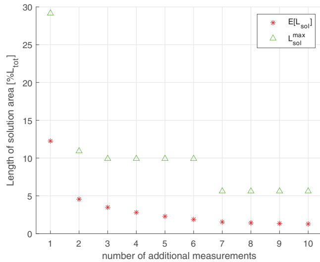
FIGURE 4 Expected and maximal value of L_{sol} for the considered 20th feeder (diamond nodes)
