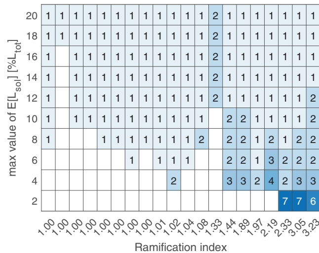
FIGURE 5 Minimum number of additional measurements needed to obtain a locating performance across the 20 reconstructed feeders ordered by ramification in columns
