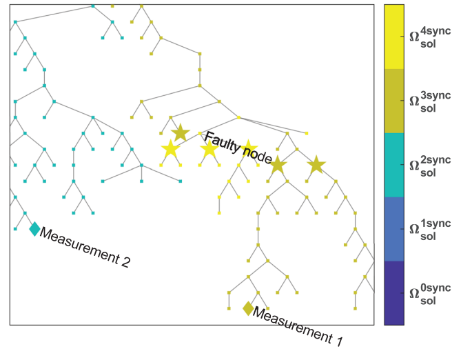
FIGURE 6 Comparison of two FLM results on the same fault with colouration by result of the presented FLM and stars for results of the Takagi method
