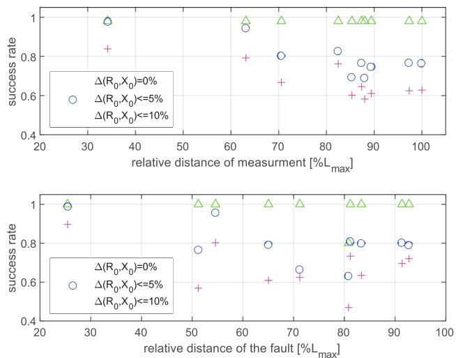
FIGURE 10 Influence of the fault and measurement positions
